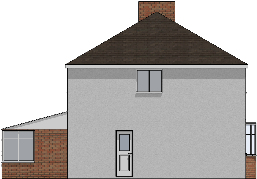
Existing Elevation - LH Side
