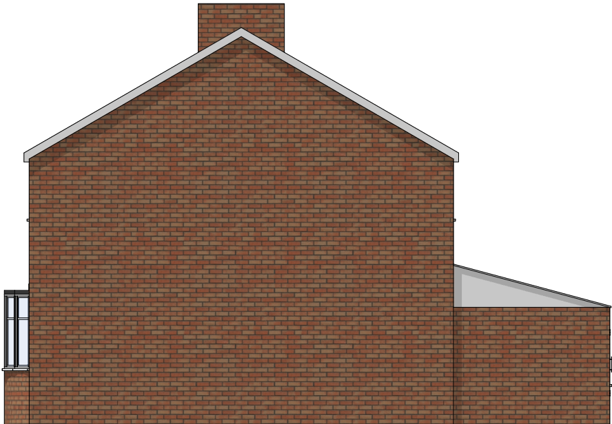
Existing Elevation - RH Side
