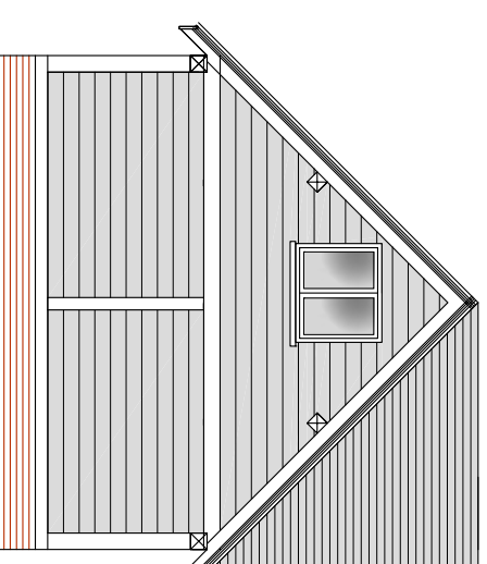
SOUTH ELEVATION
