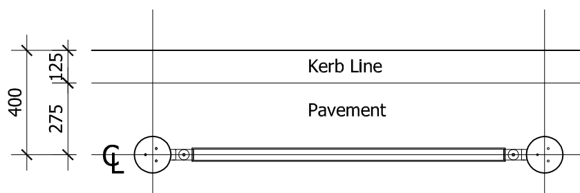
TYPICAL BARRIER OFFSET DETAIL @1:20
