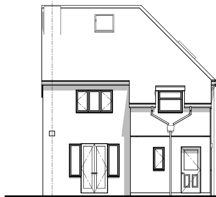
Rear Elevation
