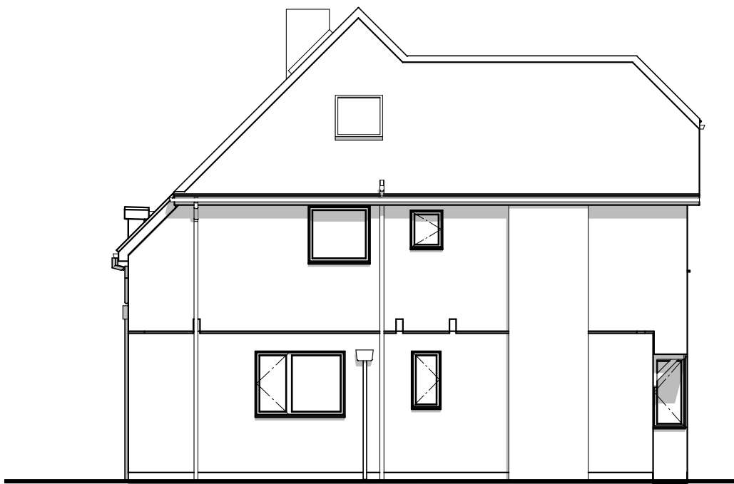
Side Elevation
