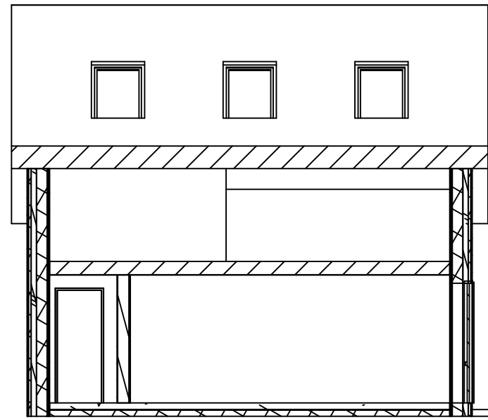
C-C Section Through (1:100)
