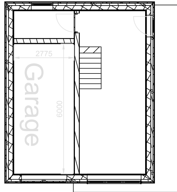
B-B Ground Level (1:100)
