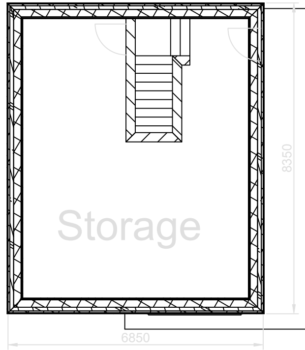
A-A Level 1 (1:100)
