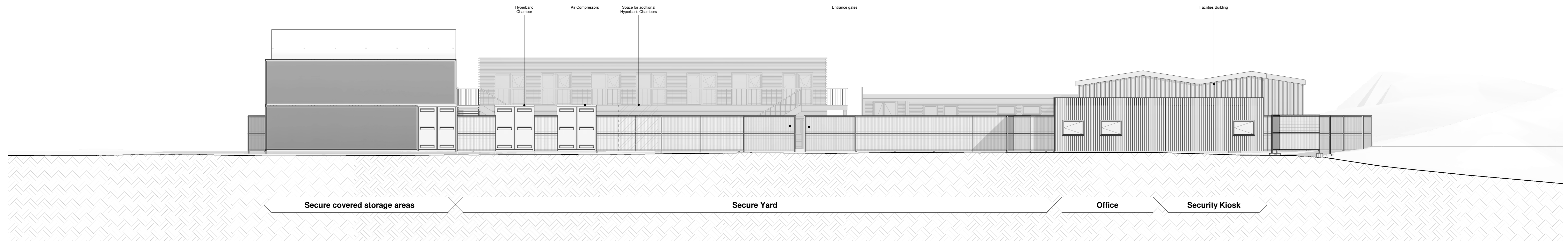
3 PL_P_231 - Operations Compound - Elevation 3 1 : 100
