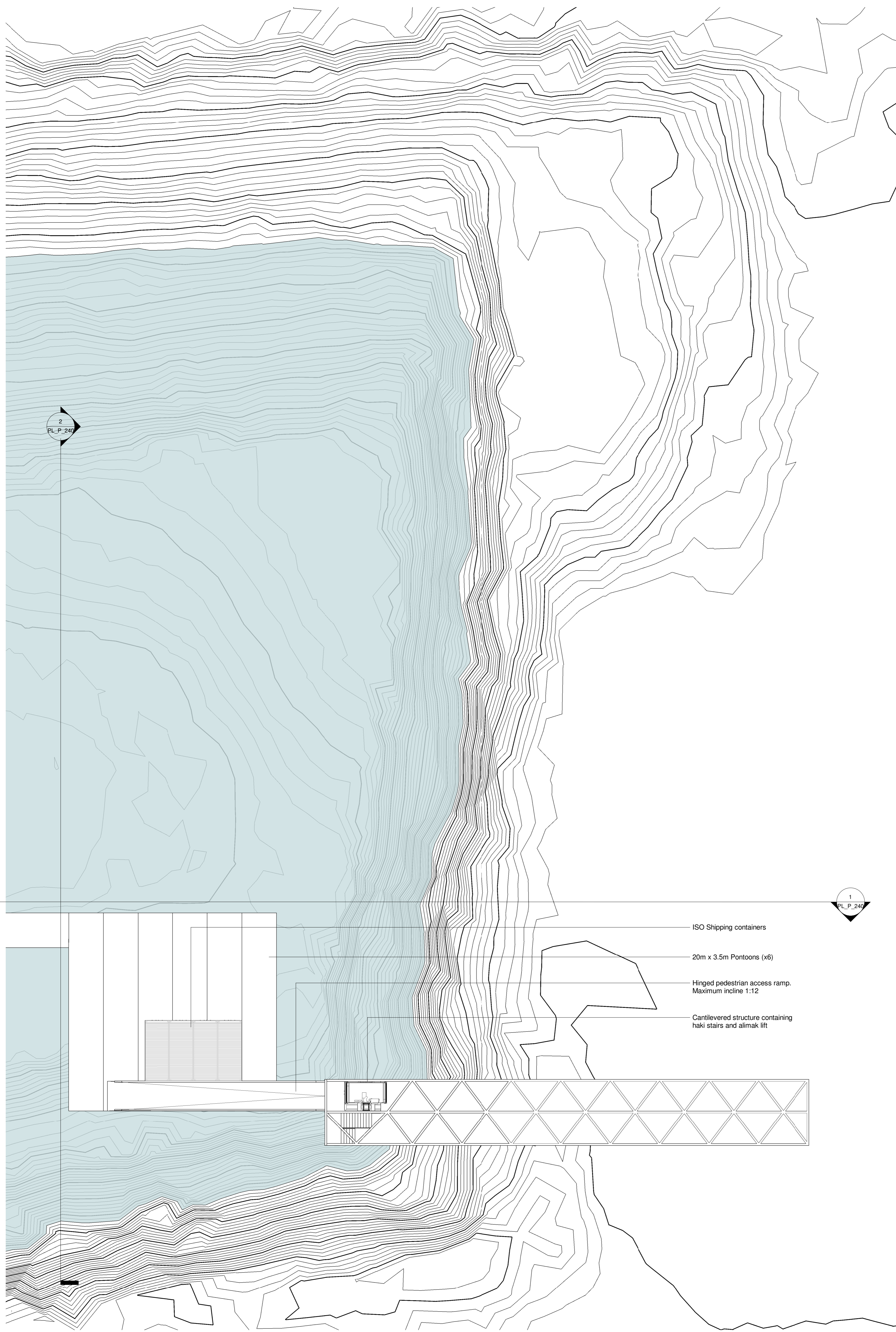
1 P - Proposed South Access 1 : 200
