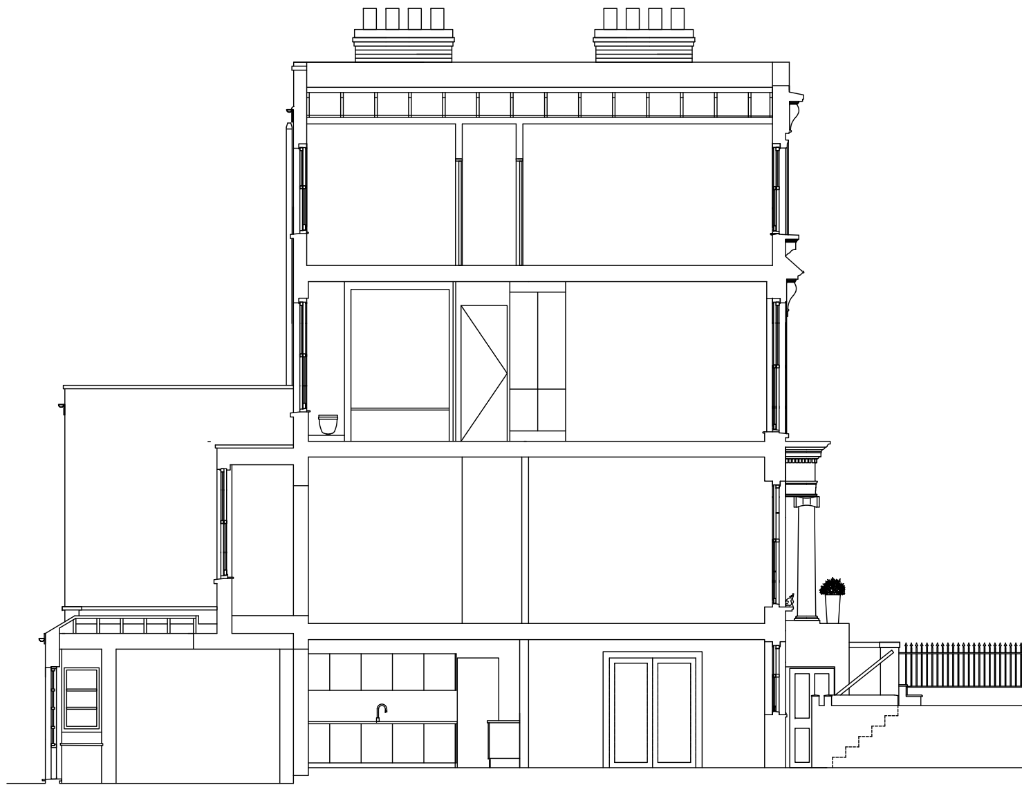
1 SECTION AA Scale @ A3, 1:100
