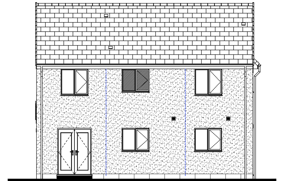
REAR ELEVATION
