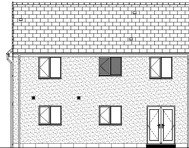
REAR ELEVATION
