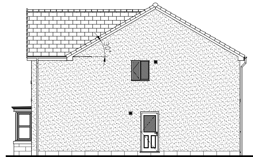
SIDE ELEVATION
