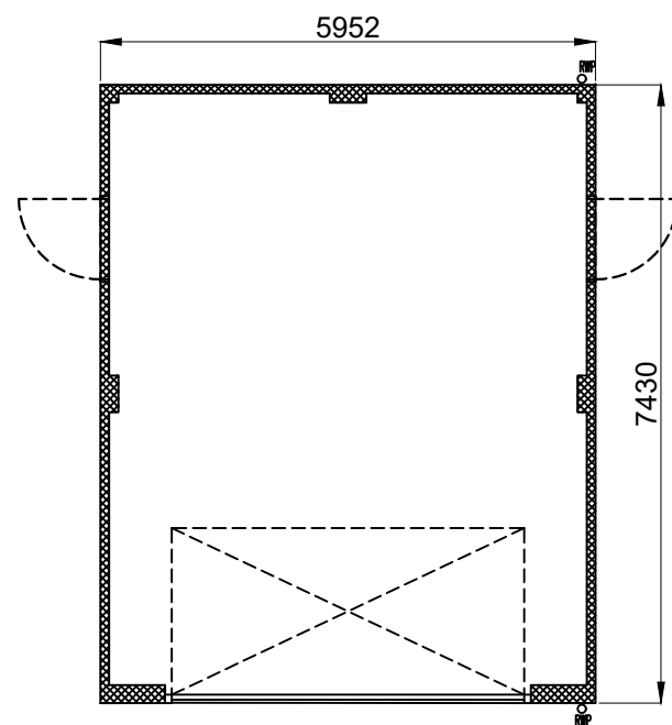
FLOOR PLAN
