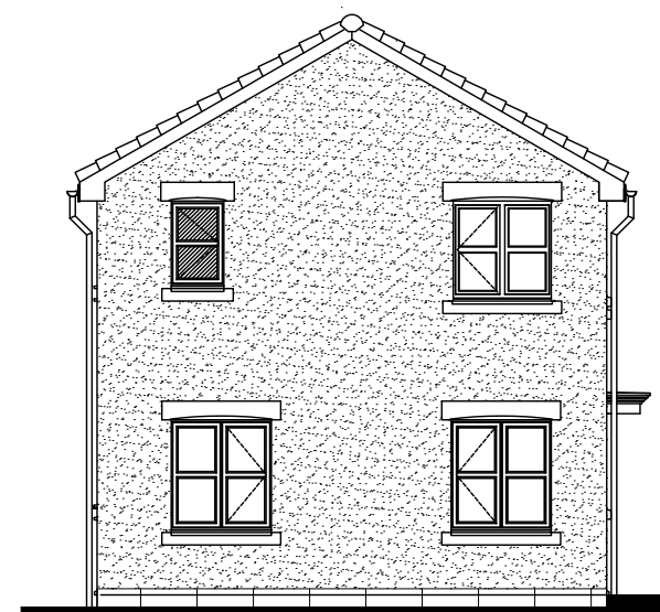
SIDE ELEVATION
