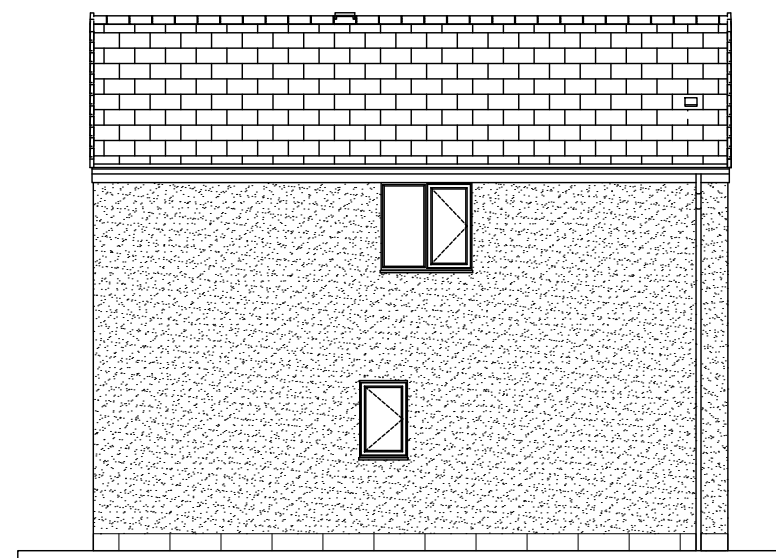
REAR ELEVATION
