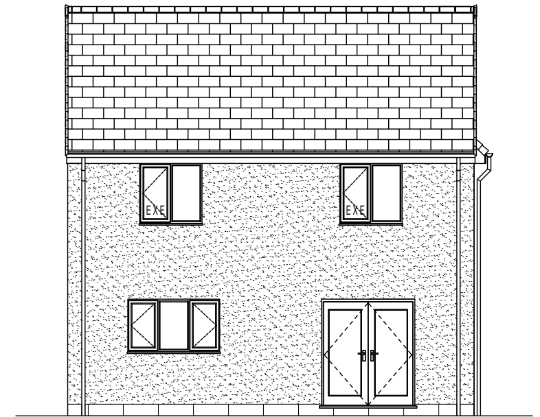
REAR ELEVATION
