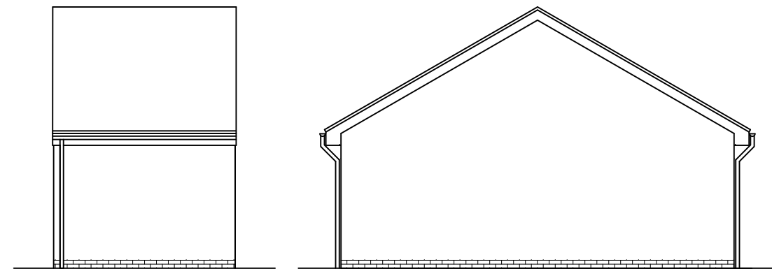
REAR ELEVATION
