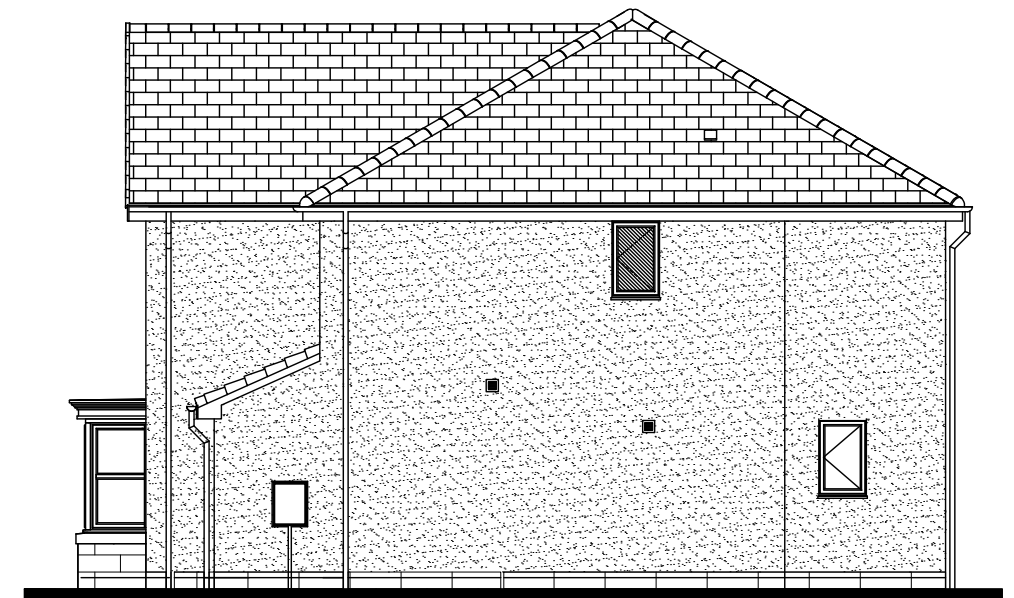
SIDE ELEVATION
