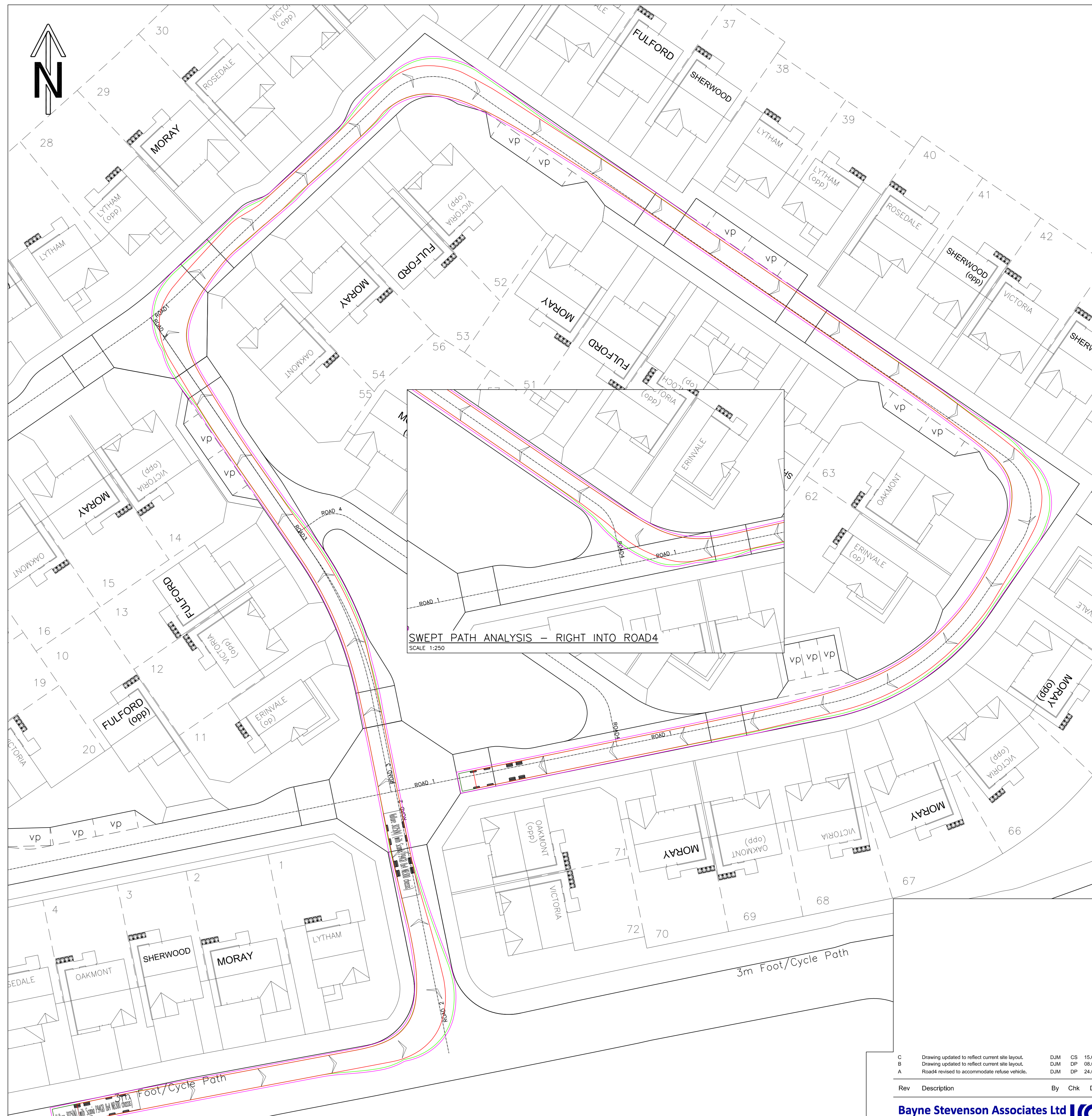
SWEPT PATH ANALYSIS - TRACK 2 SCALE 1:250
