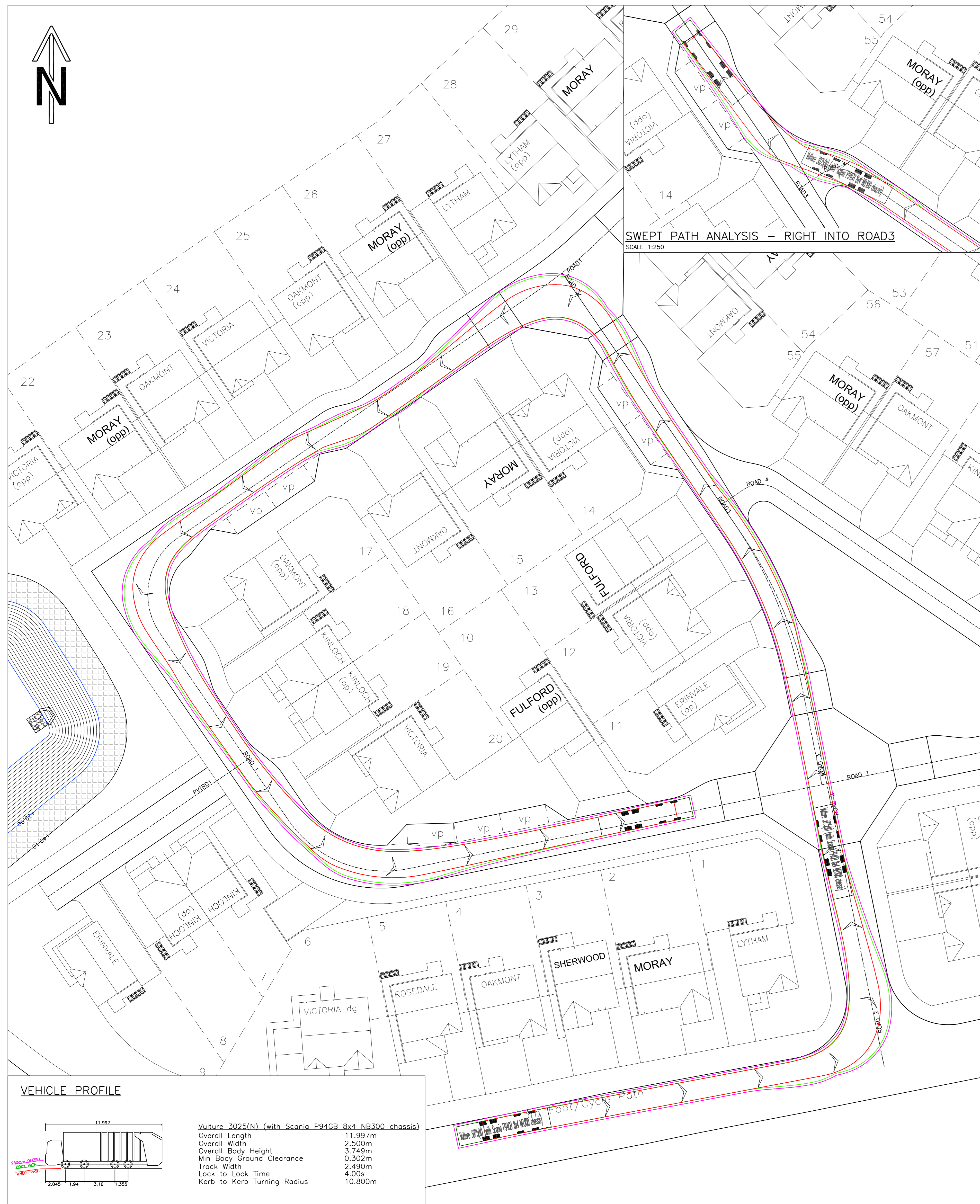
SWEPT PATH ANALYSIS - TRACK 1 SCALE 1:250
