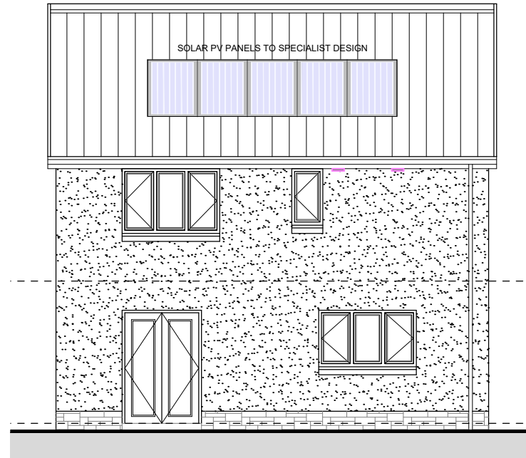
Rear Elevation
