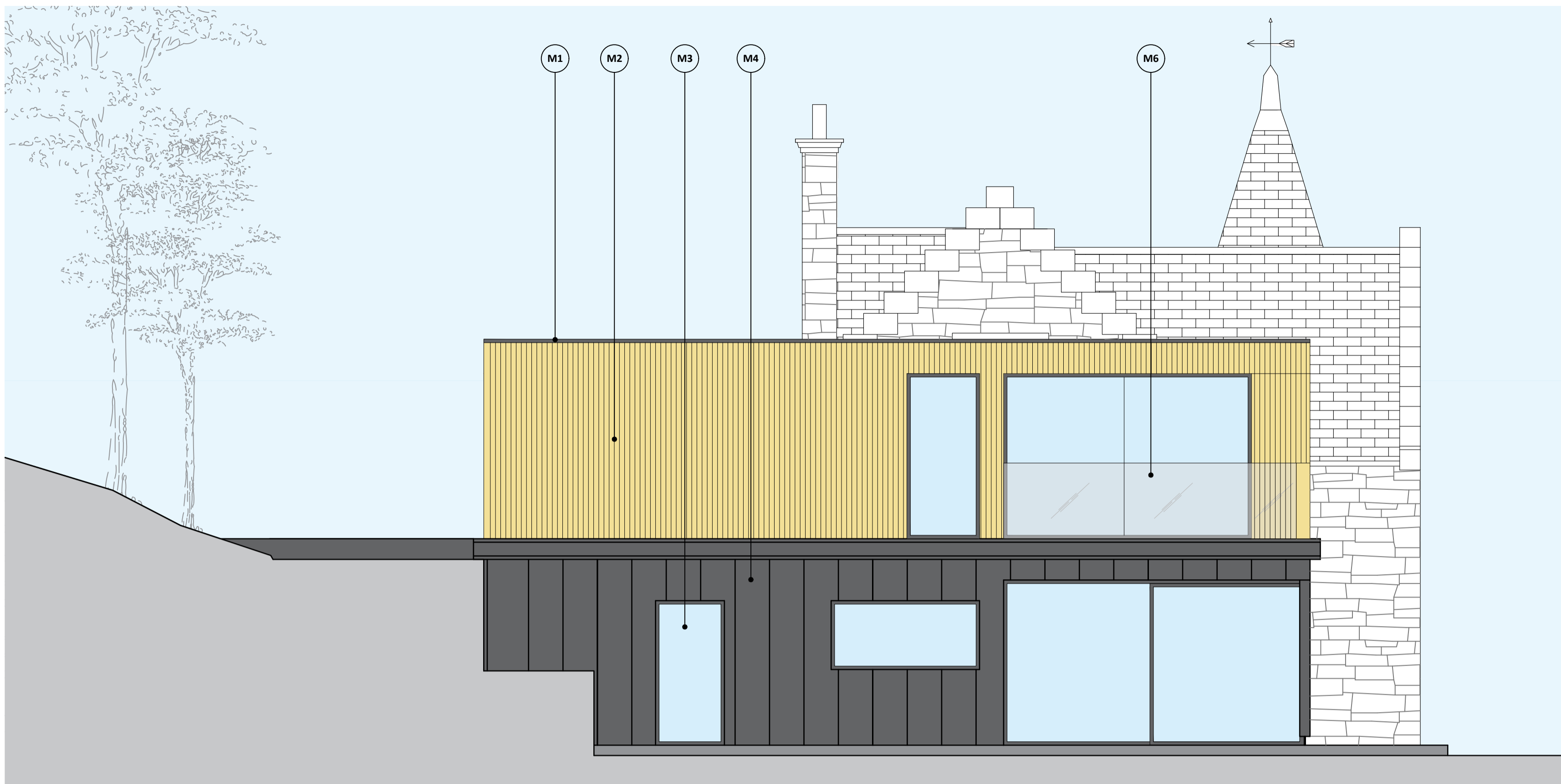
Proposed Side Elevation (E3)
