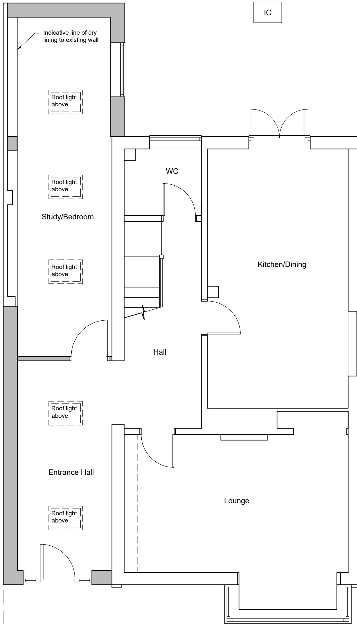
1. Proposed Ground Floor plan 1:50@A3
