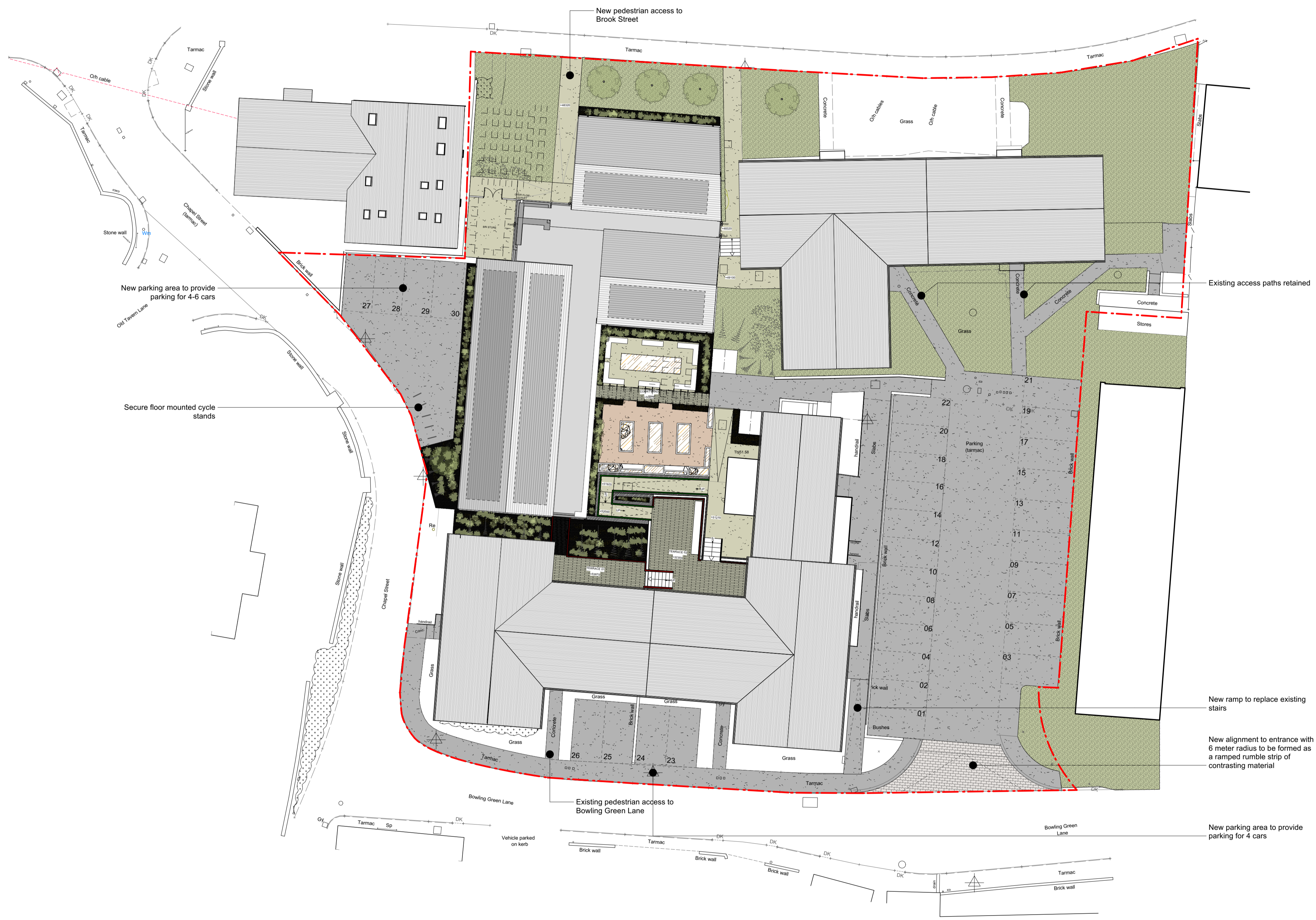
GA.201.2 SITE PLAN AS PROPOSED SCALE 1:200 @ A1, 1:400 @ A3
