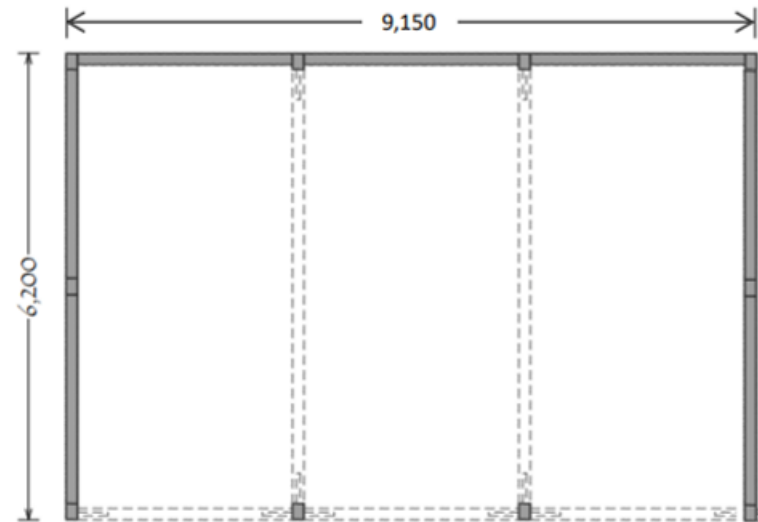
FLOOR PLAN
