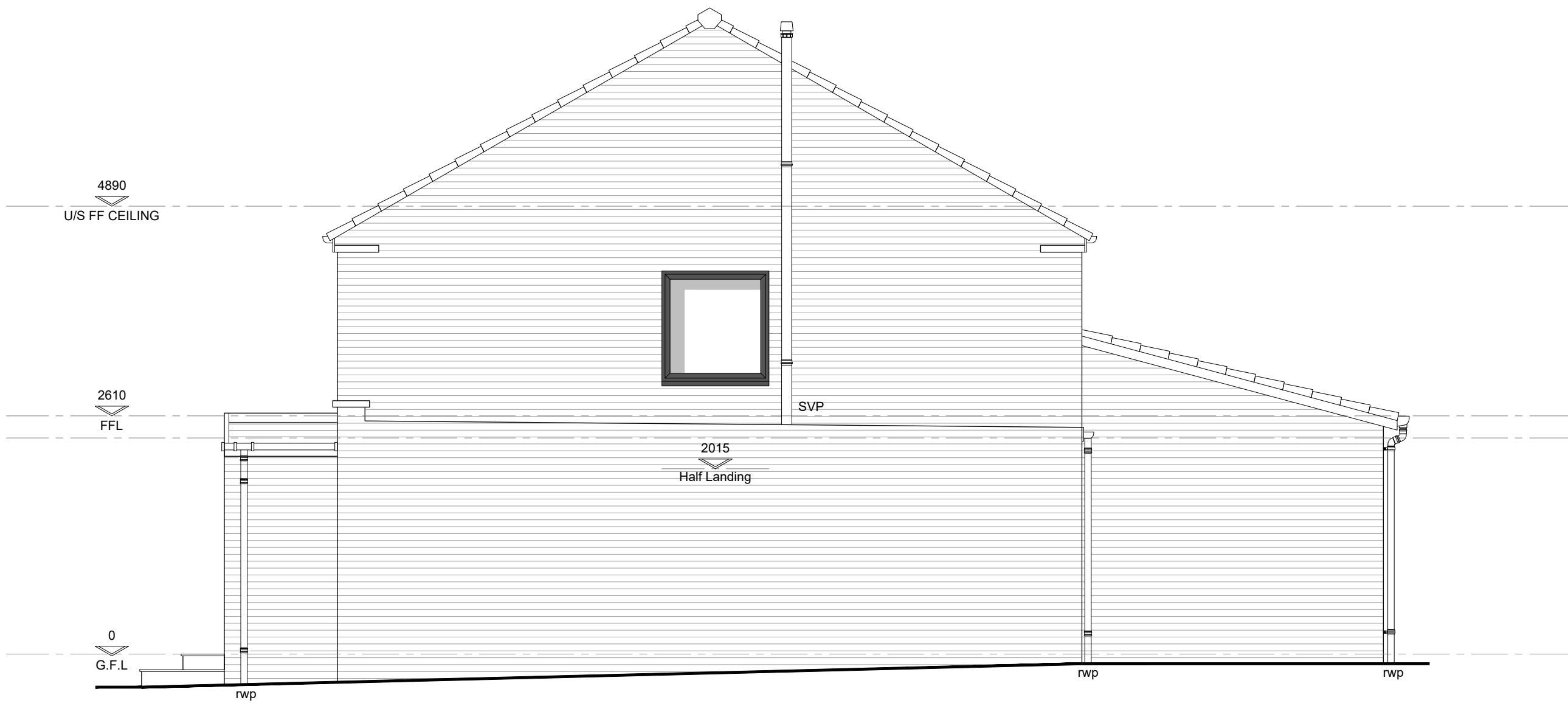
EXISTING SIDE ELEVATION (SOUTH) Scale 1:50
