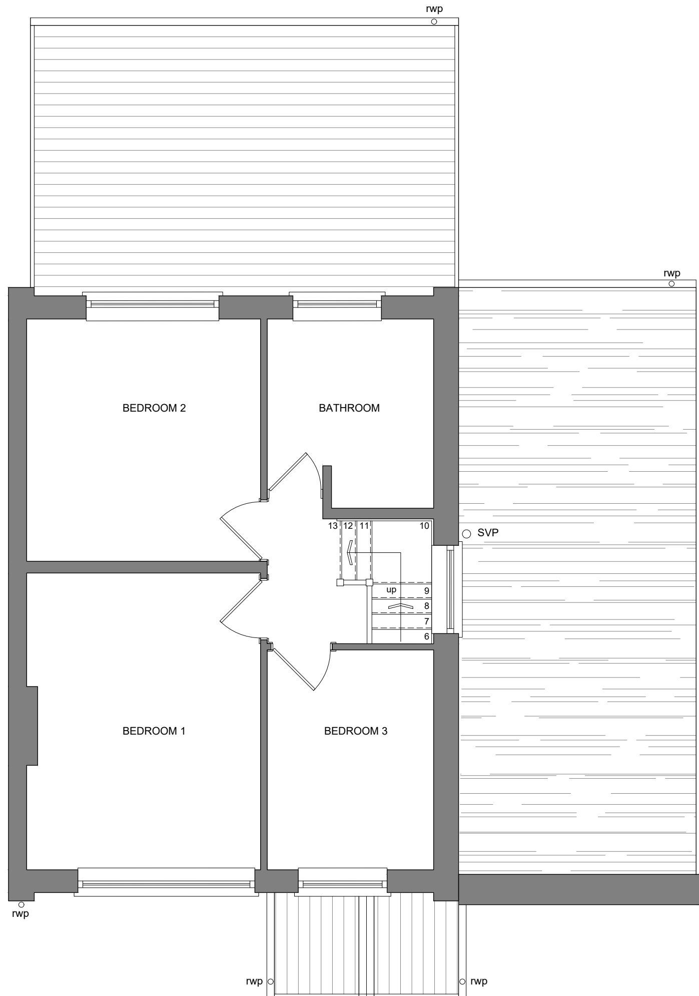
EXISTING FIRST FLOOR PLAN Scale 1:50
