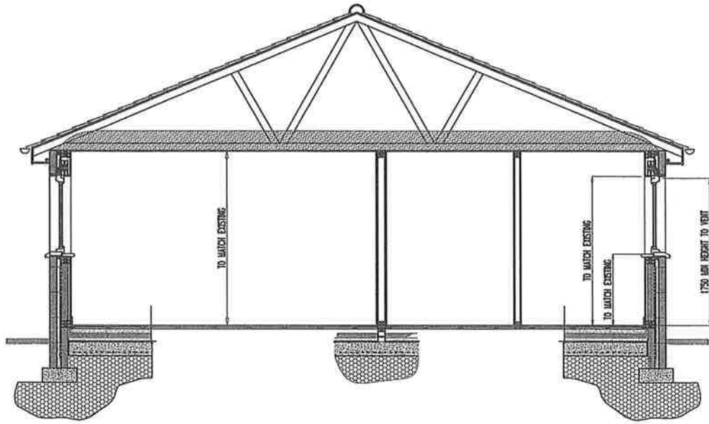
CROSS SECTION AS PROPOSED
