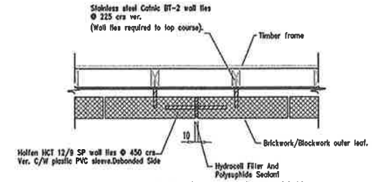
MOVEMENT JOINT DETAIL AT MID SPAN LONG EXTERNAL WALL
