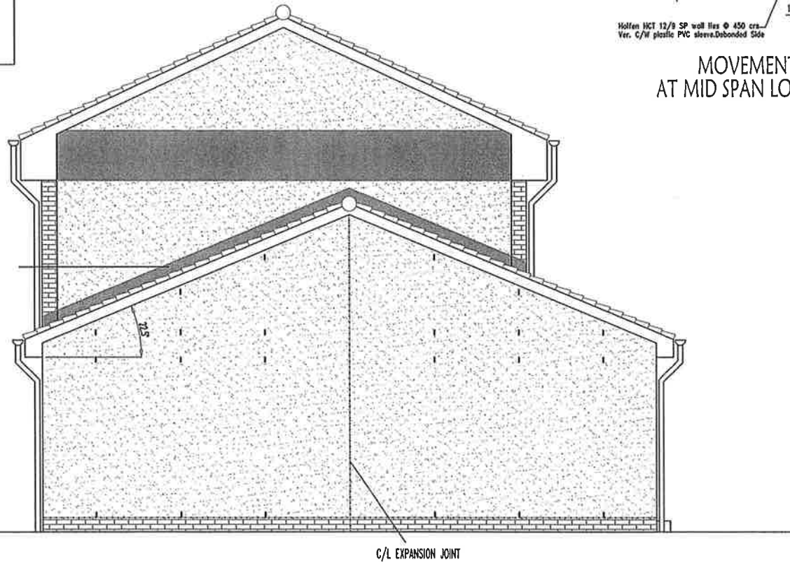
GABLE ELEVATION AS PROPOSED
