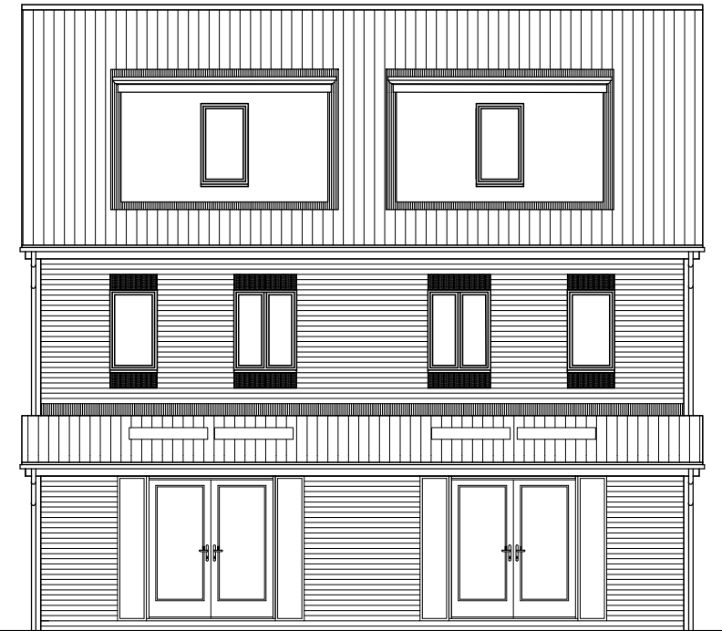
REAR ELEVATION
