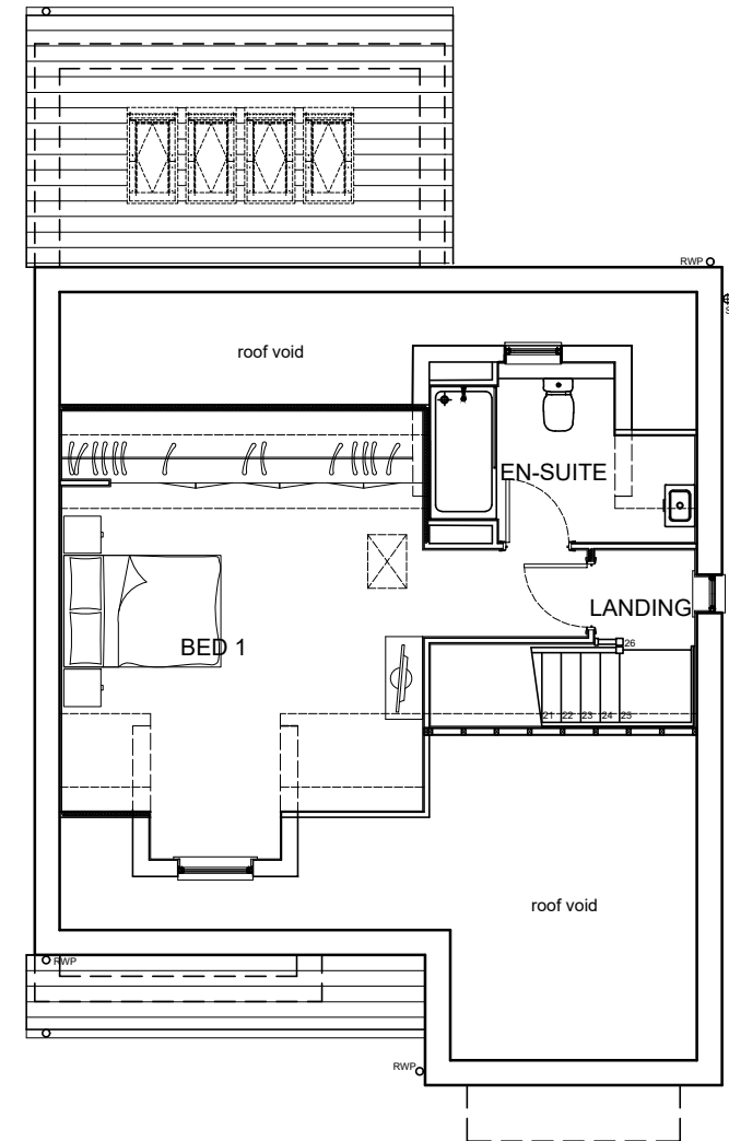
SECOND FLOOR
