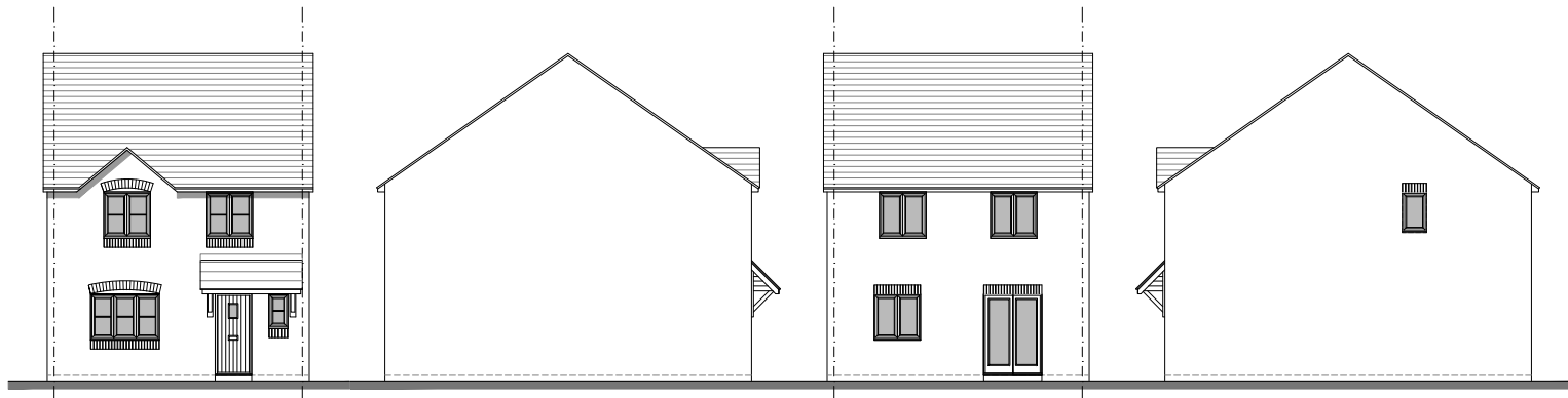
ELEVATIONS (1:200)
