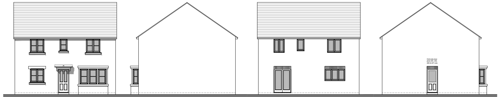
ELEVATIONS (1:200)
