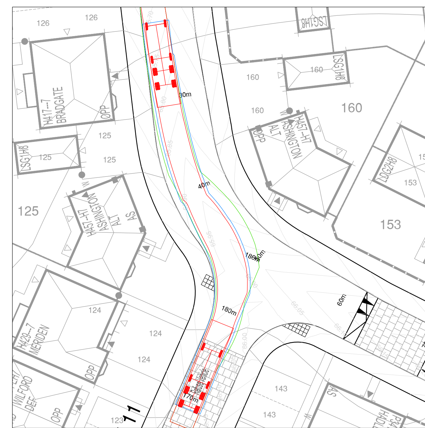
Right Turn - Road 11 to Road 10
