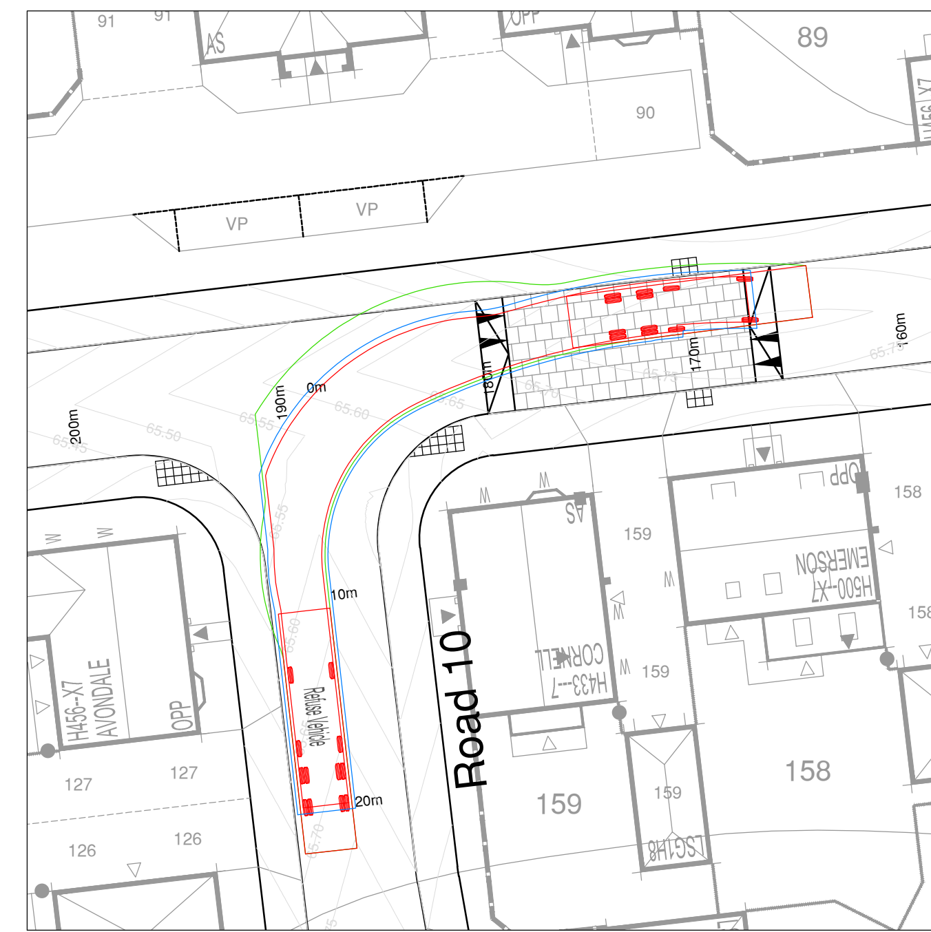
Right Turn - Road 10 to Road 8
