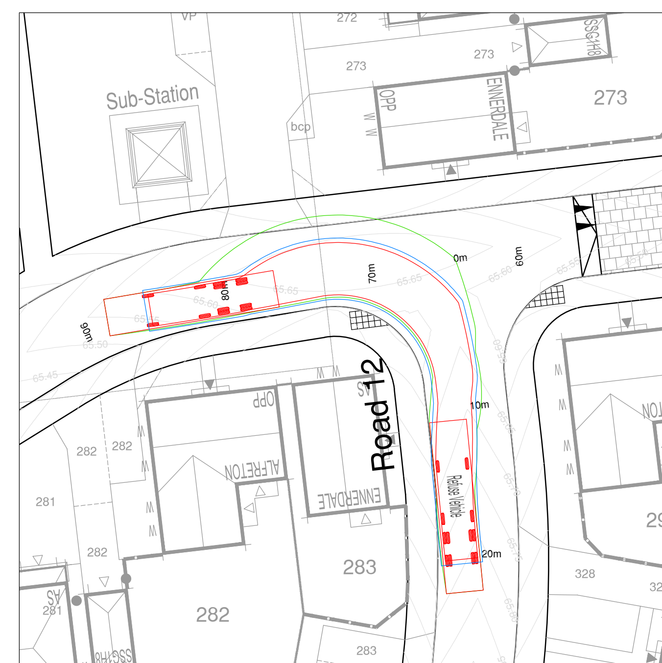
Left Turn - Road 12 to Road 7
