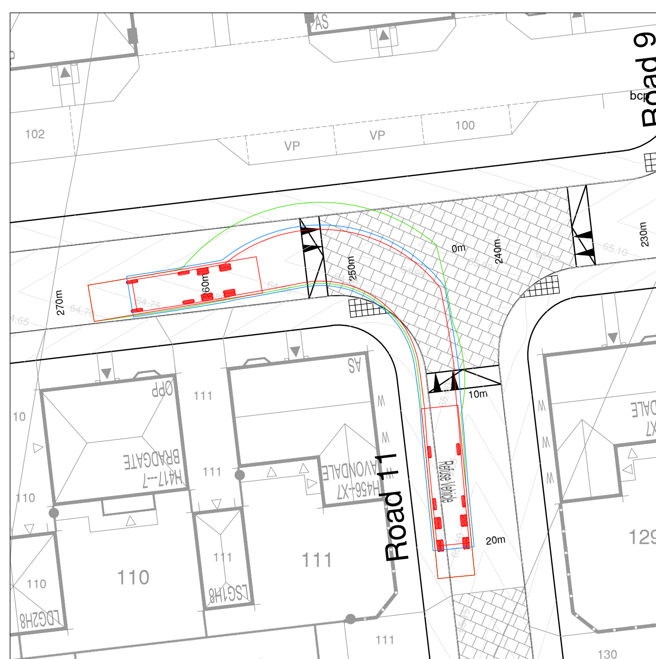
Left Turn - Road 11 to Road 8
