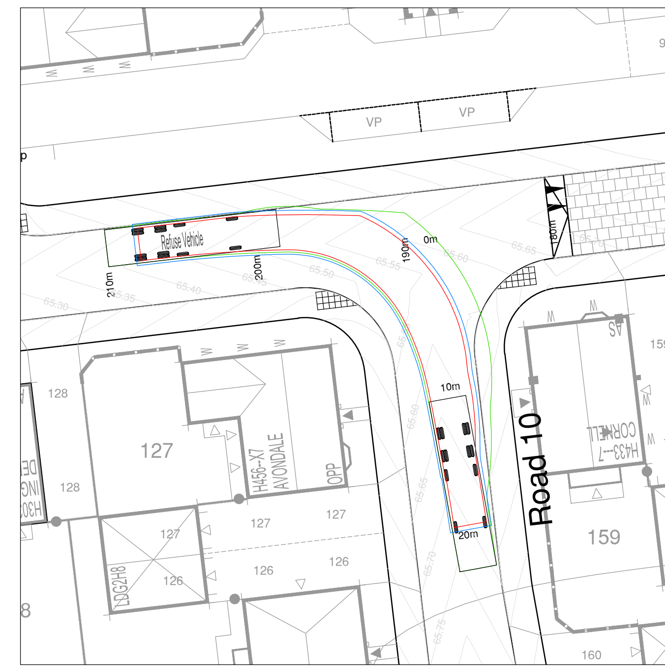
Right Turn - Road 8 to Road 10
