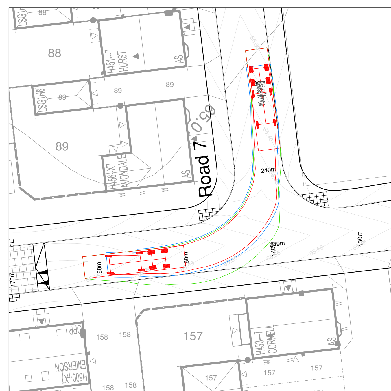
Right Turn - Road 7 to Road 8
