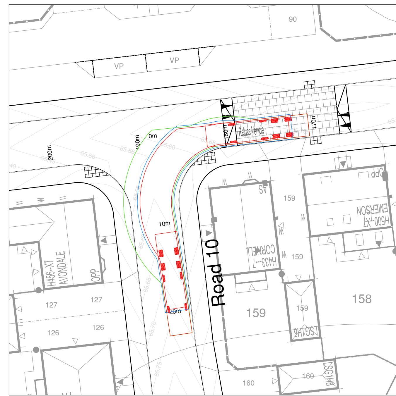
Left Turn - Road 8 to Road 10
