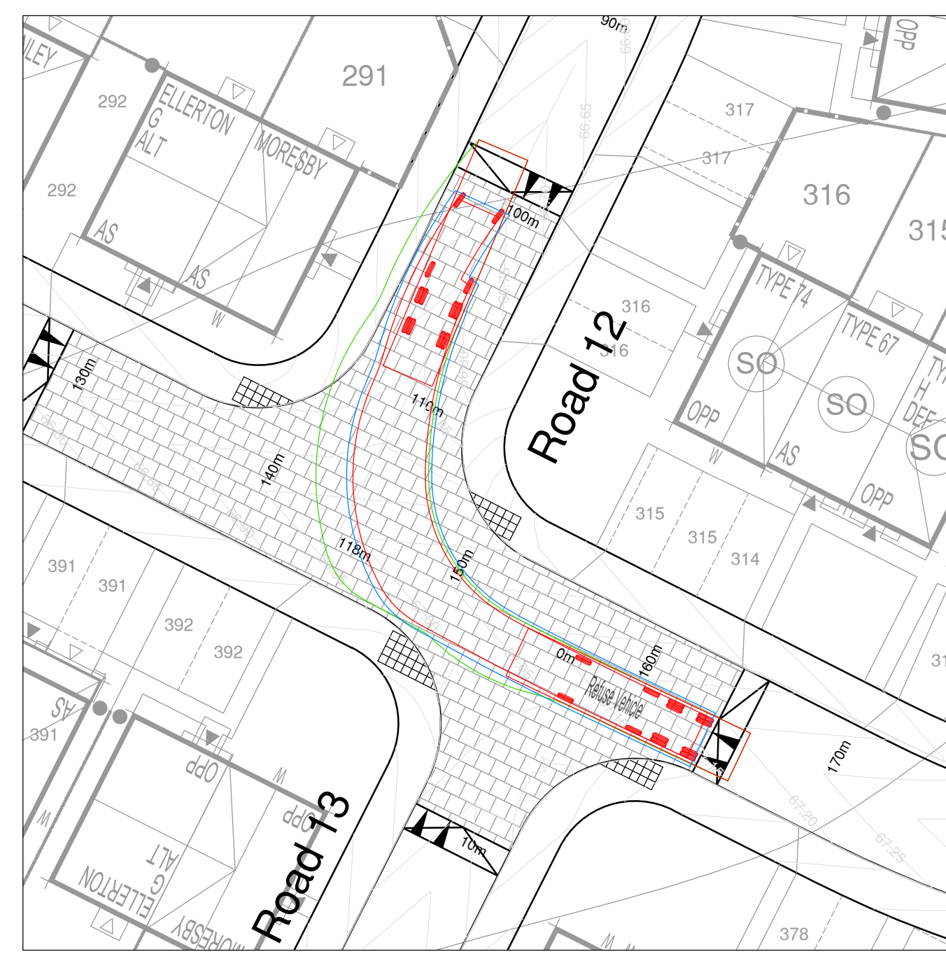
Right Turn - Road 10 to Road 12
