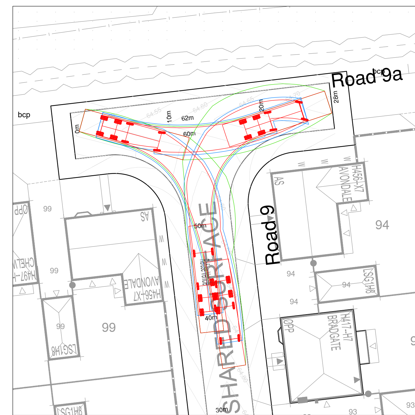
Turning Head - Road 9a
