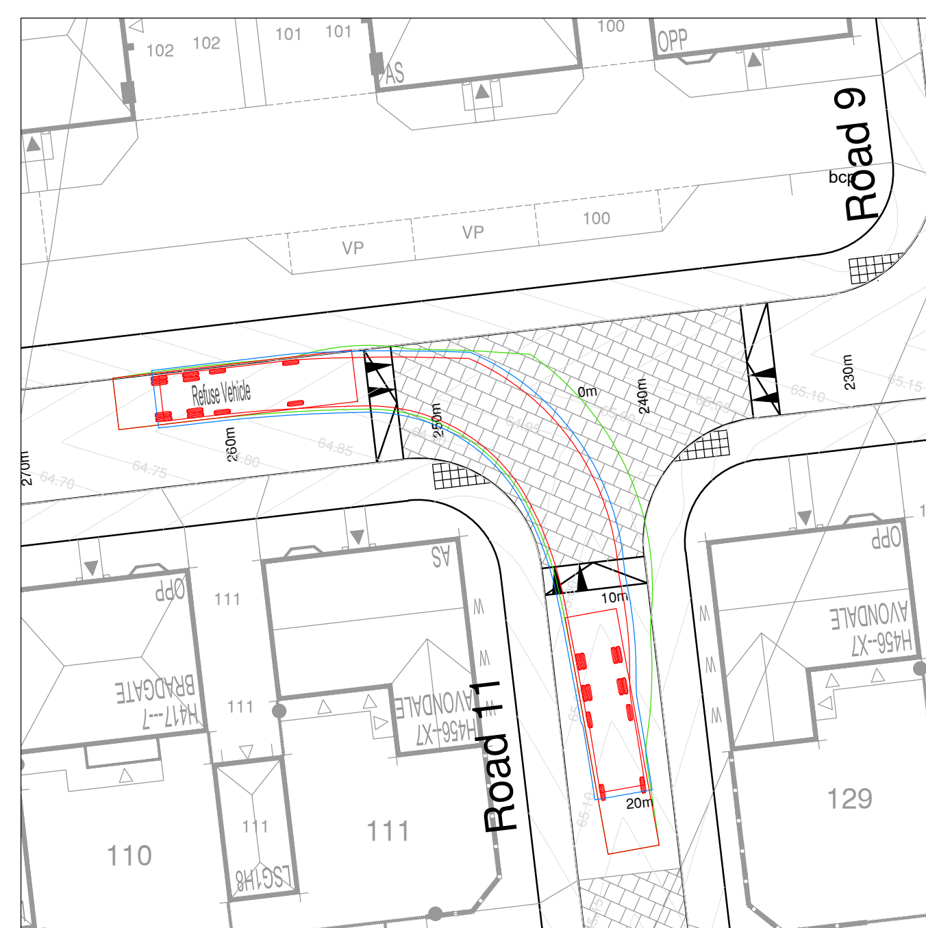
Right Turn - Road 8 to Road 11
