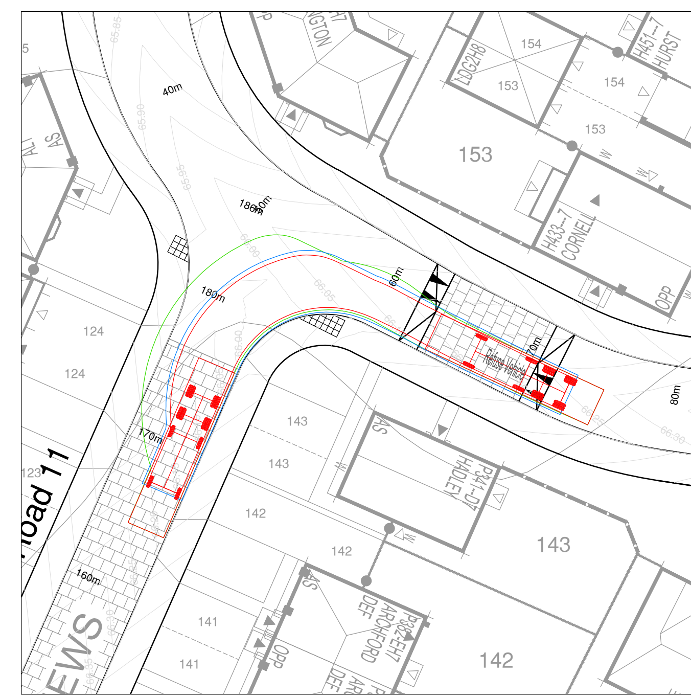
Left Turn - Road 10 to Road 11
