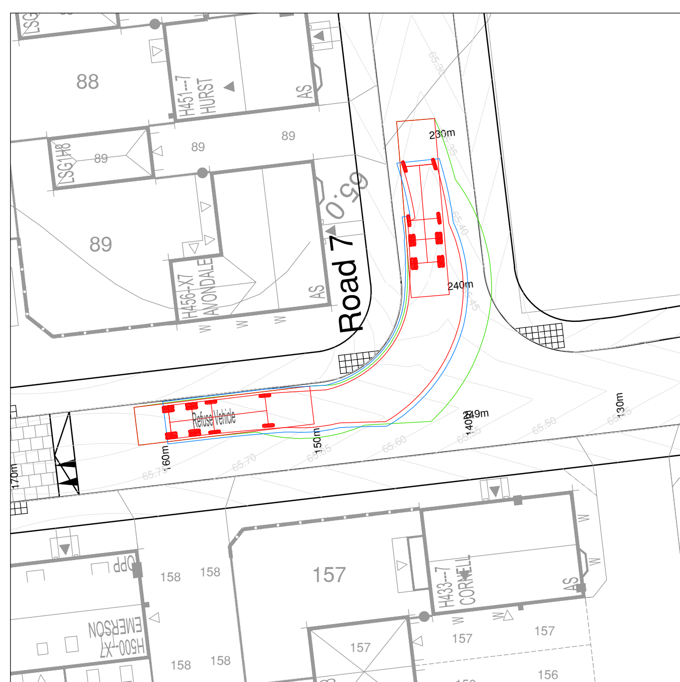
Left Turn - Road 8 to Road 7
