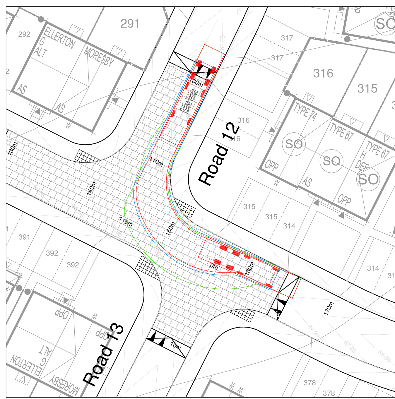
Left Turn - Road 12 to Road 10
