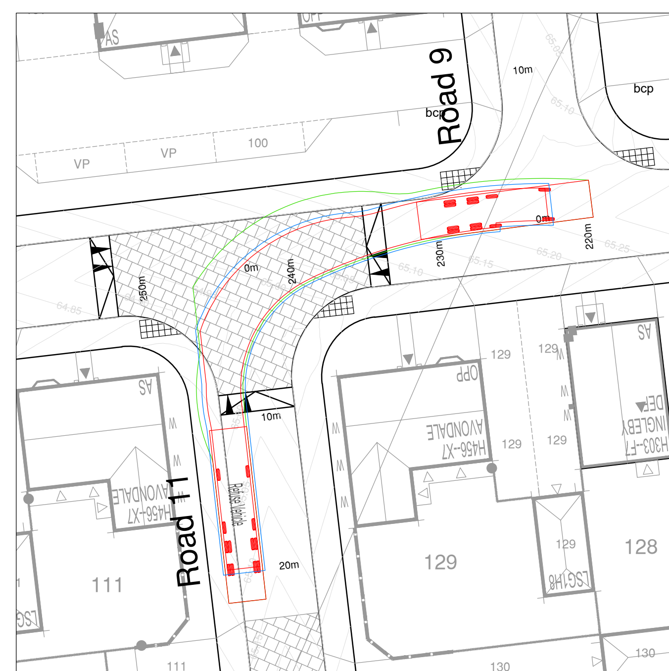
Right Turn - Road 11 to Road 8
