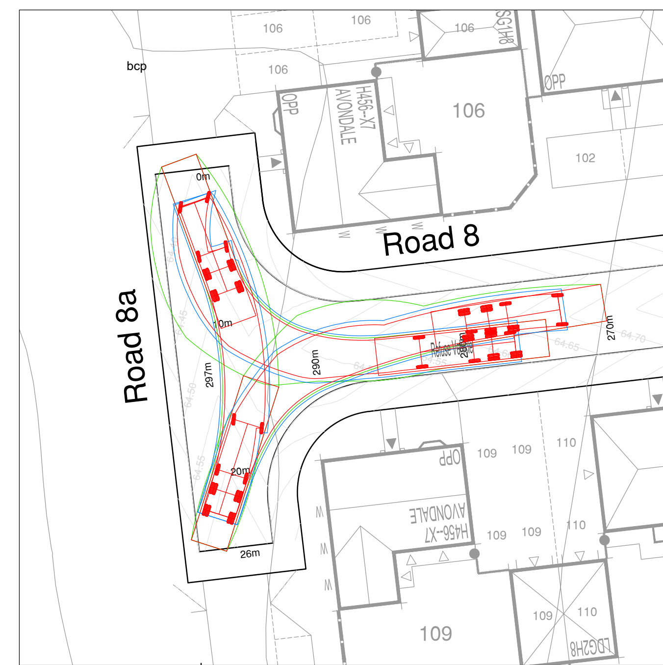
Turning Head - Road 8a
