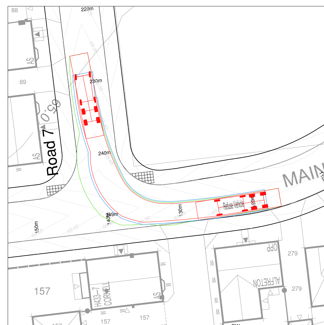
Right Turn - Road 8 to Road 7
