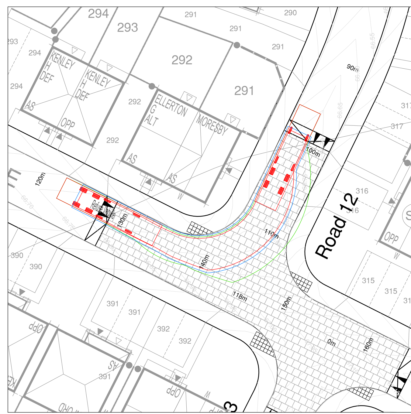
Left Turn - Road 10 to Road 12
