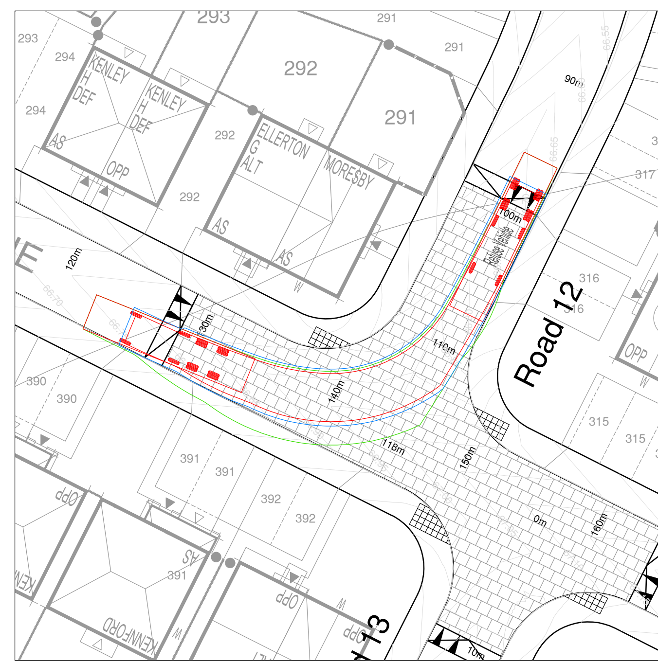
Right Turn - Road 12 to Road 10
