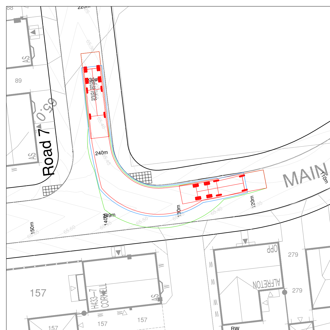
Left Turn - Road 7 to Road 8
