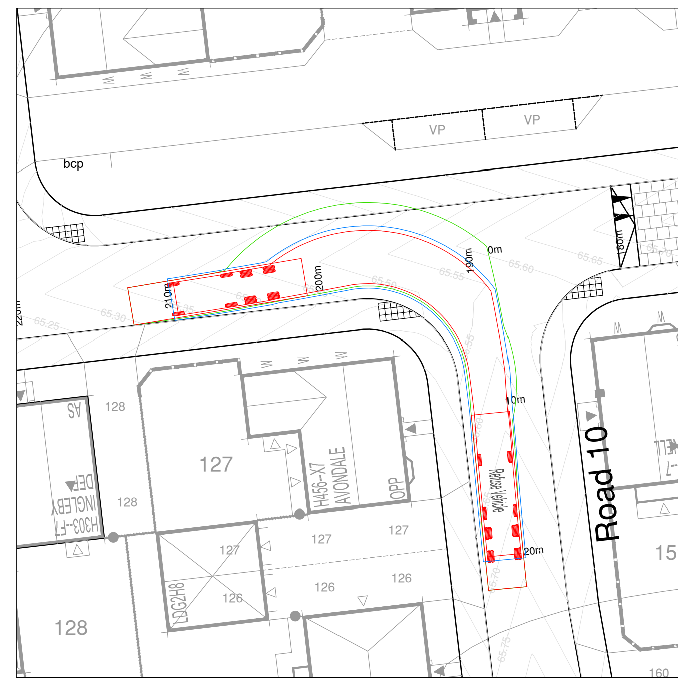
Left Turn - Road 10 to Road 8
