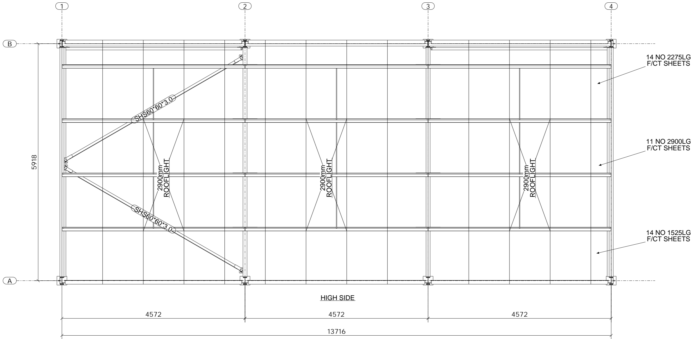
ROOF PLAN VIEW
