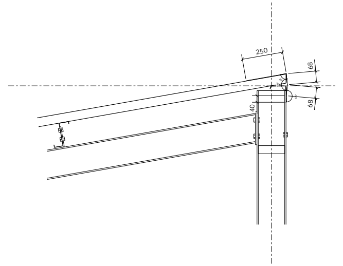
RIDGE FLASHING
