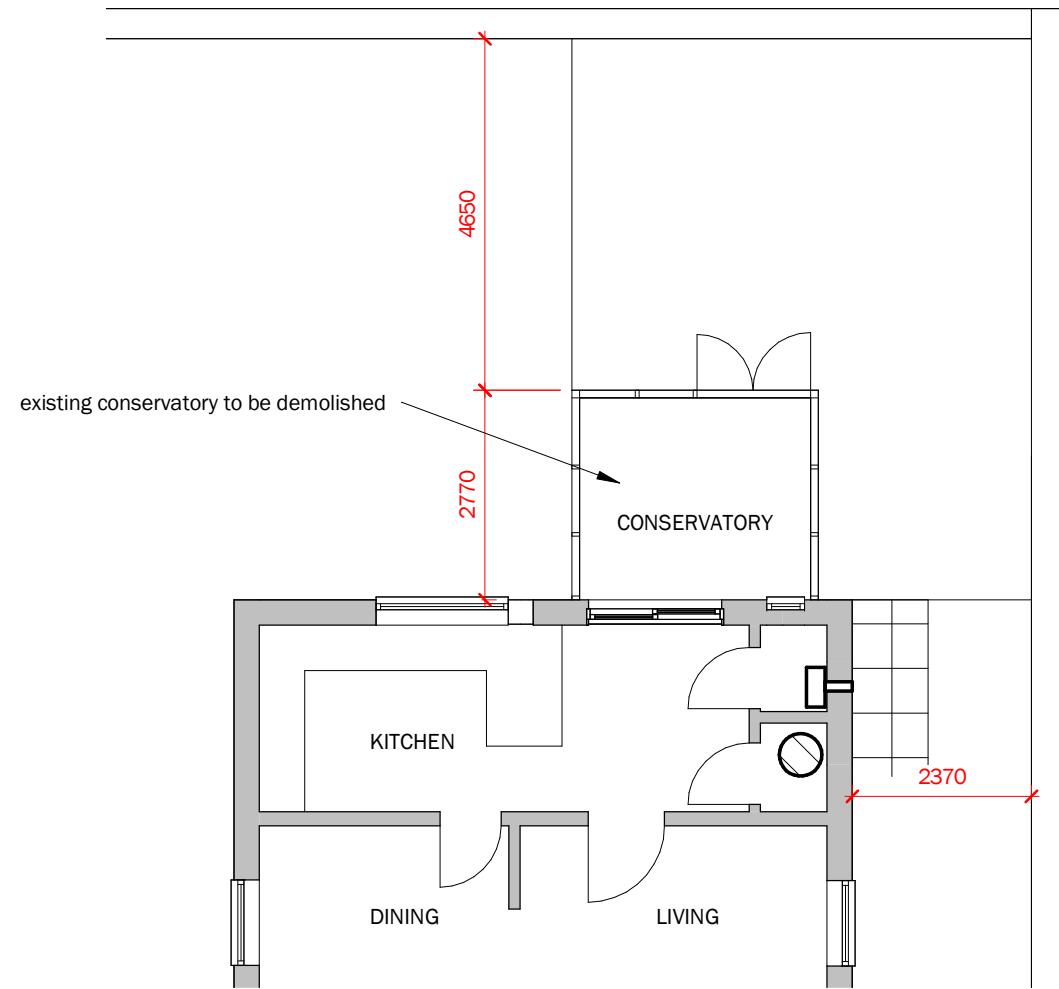
Ground Floor - Existing 1 : 100
