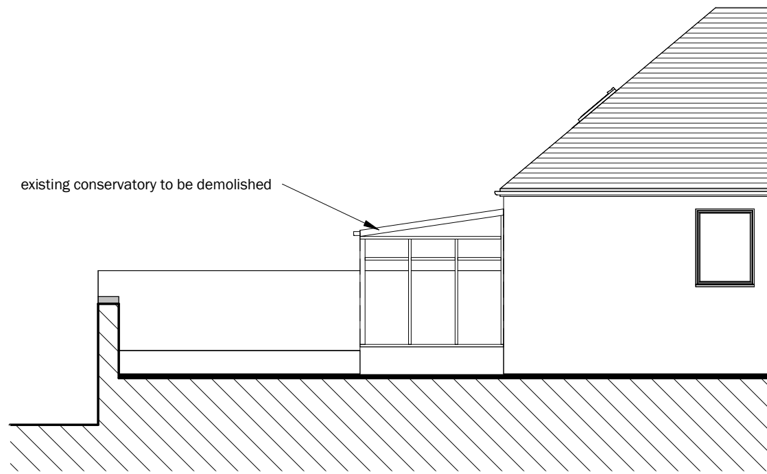
S Elevation - Existing 1 : 100
