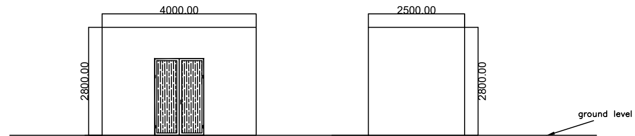
external elevation wall 3 external elevation wall 4
