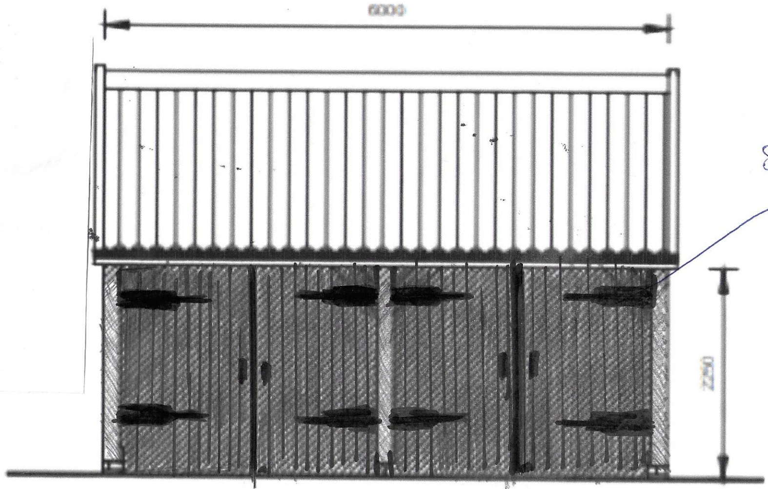
FRONT ELEVATION 1:100
