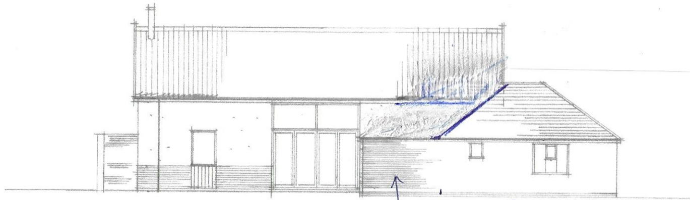
SOUTH ELEVATION
