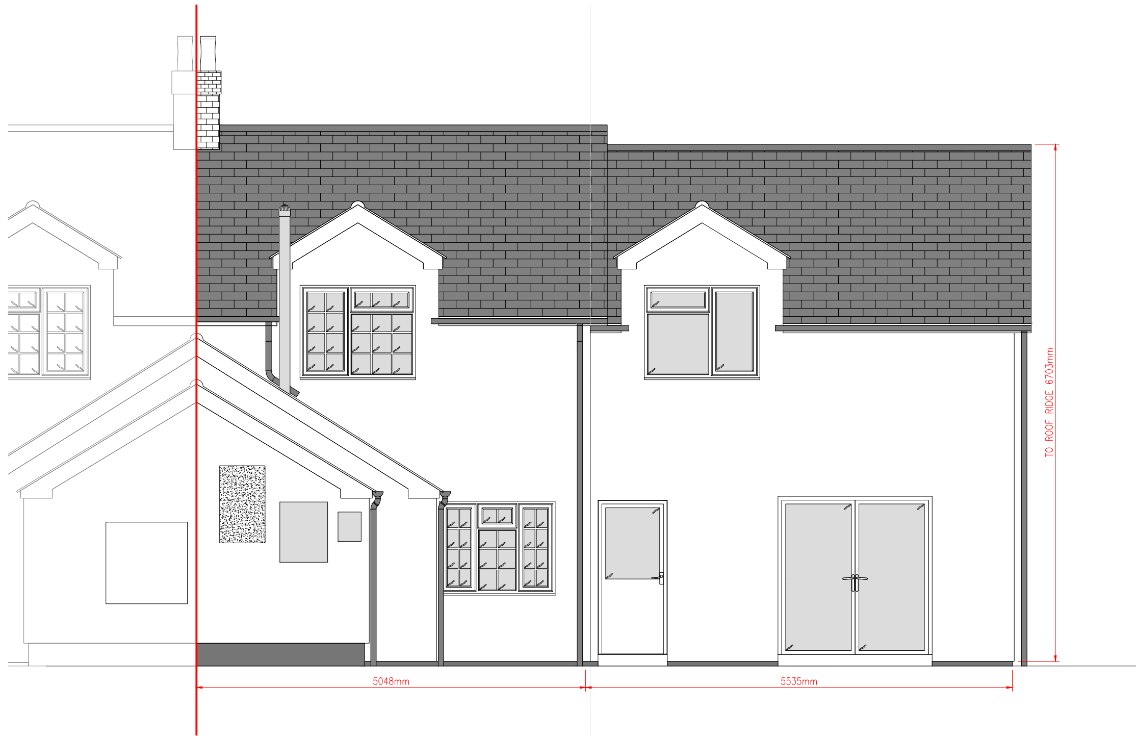
North Elevation
