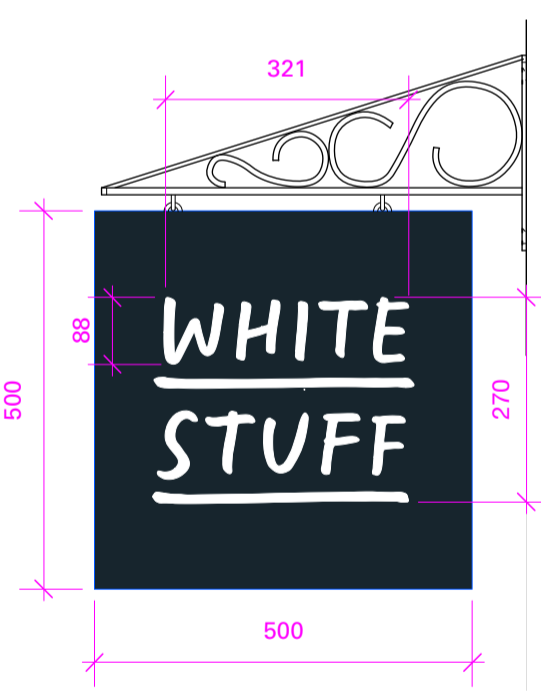
PROPOSED HANGING SIGN 1:10
