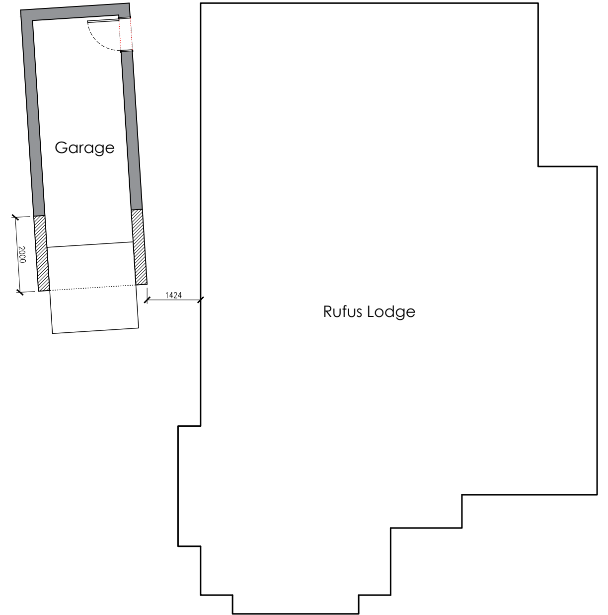
Proposed Garage Floor Plan 1:100
