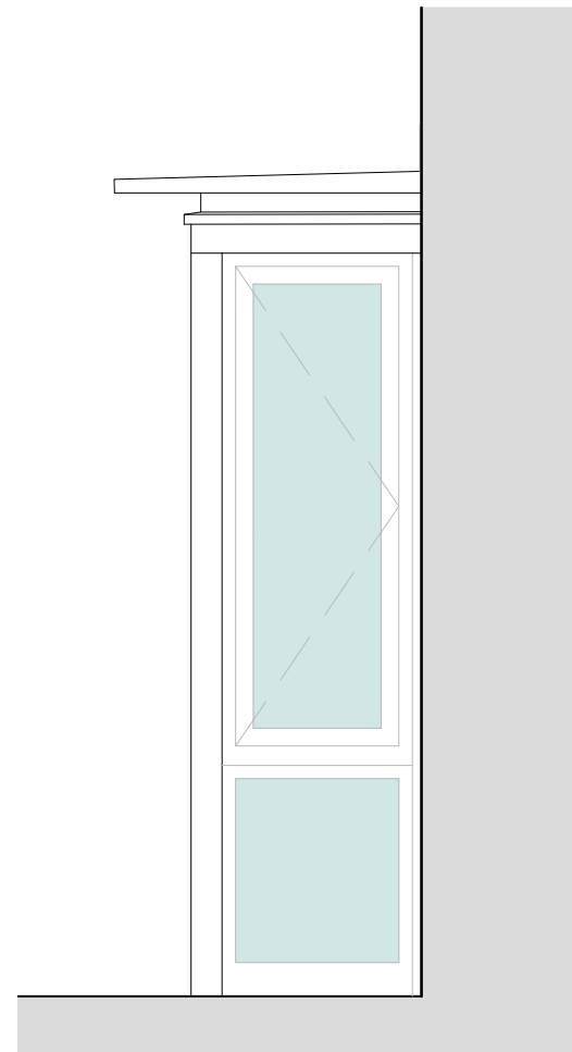
Bay Window Side Elevation: 1:25 scale @ A3
