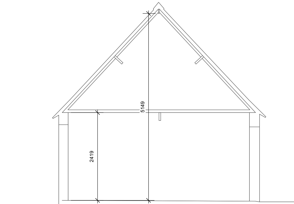
EXISTING SECTION THROUGH GARAGE
