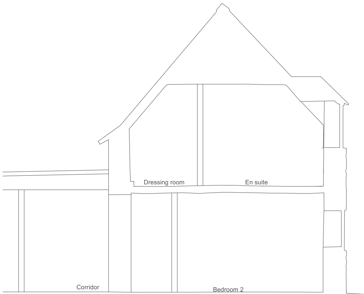
SECTION B-B (through dressing room and en suite)
