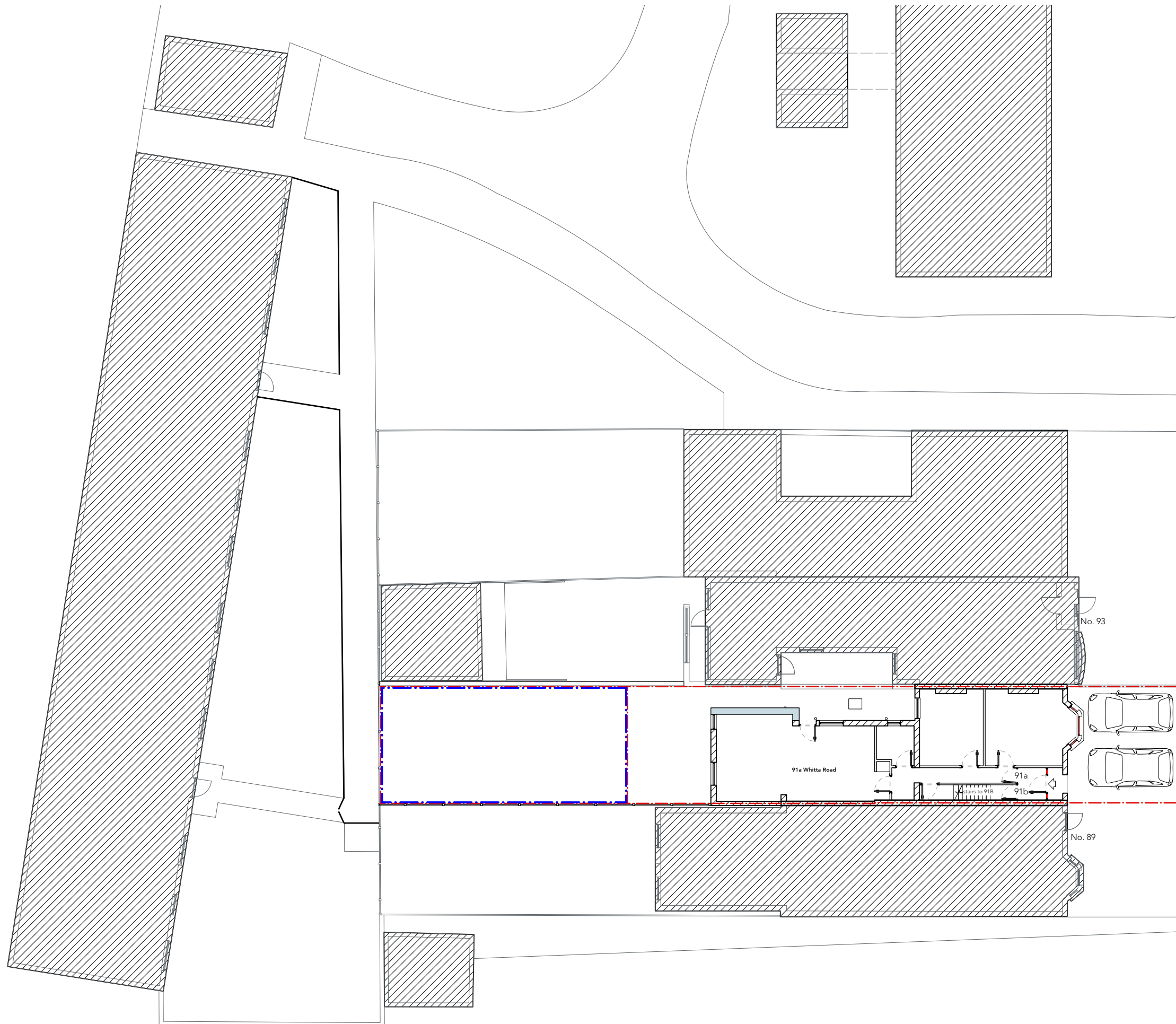
BLOCK PLAN / GROUND FLOOR - 91A WHITTA ROAD
