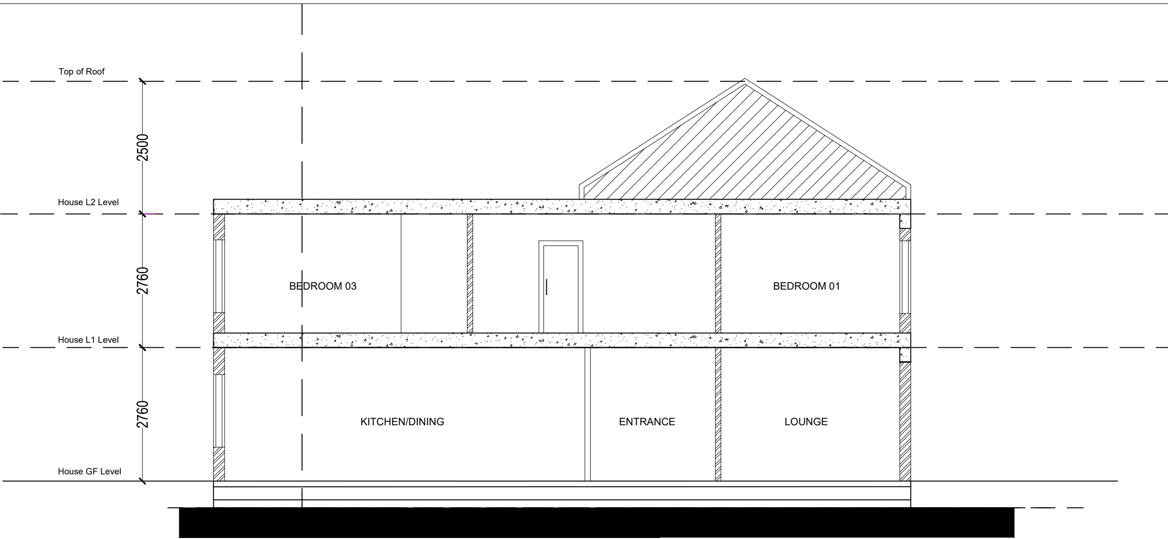
Proposed Section _ SECION THRO AA-AA'
