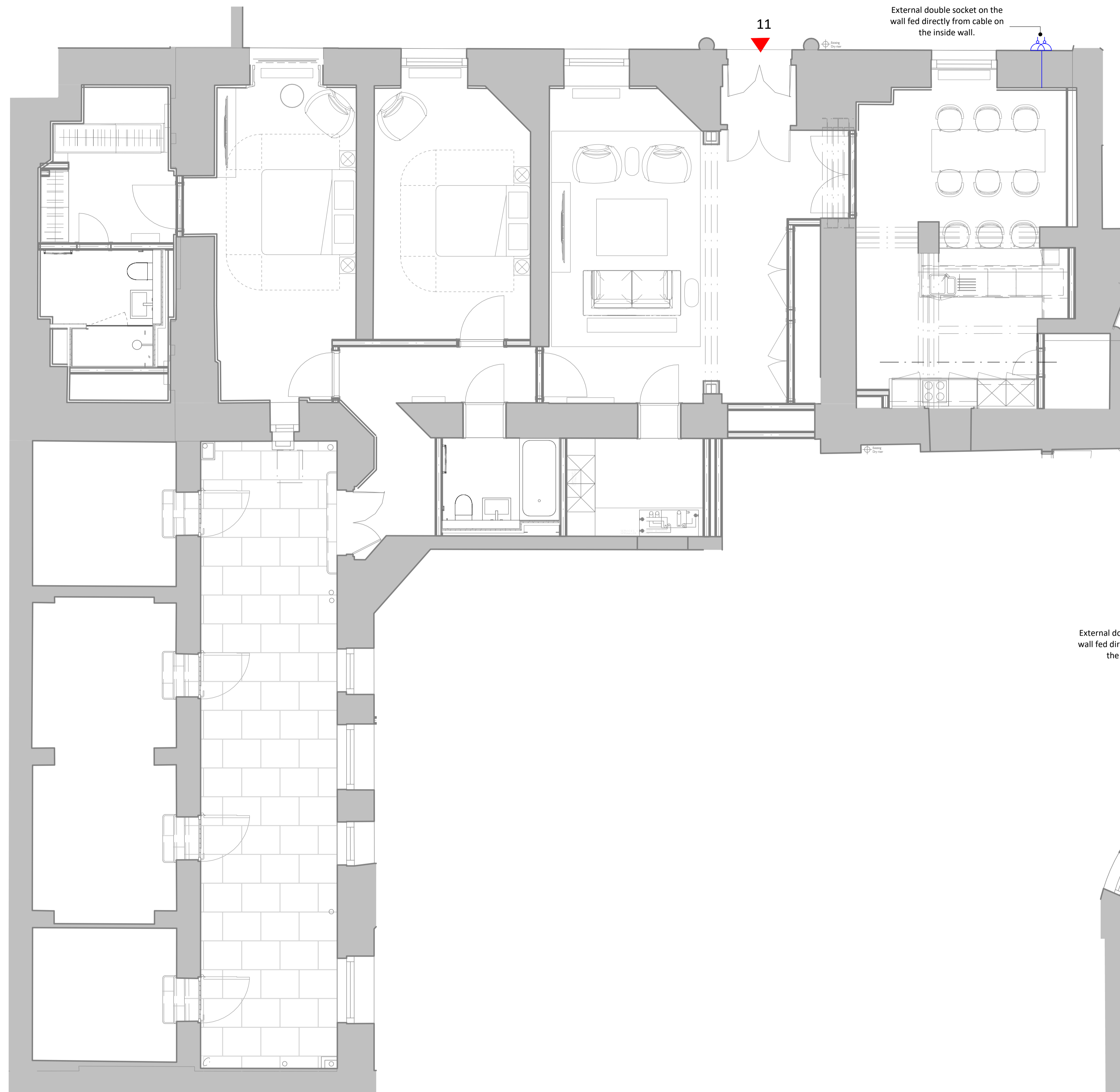
1 FT11 - LGF - Proposed Small Power Plan 1 : 50
