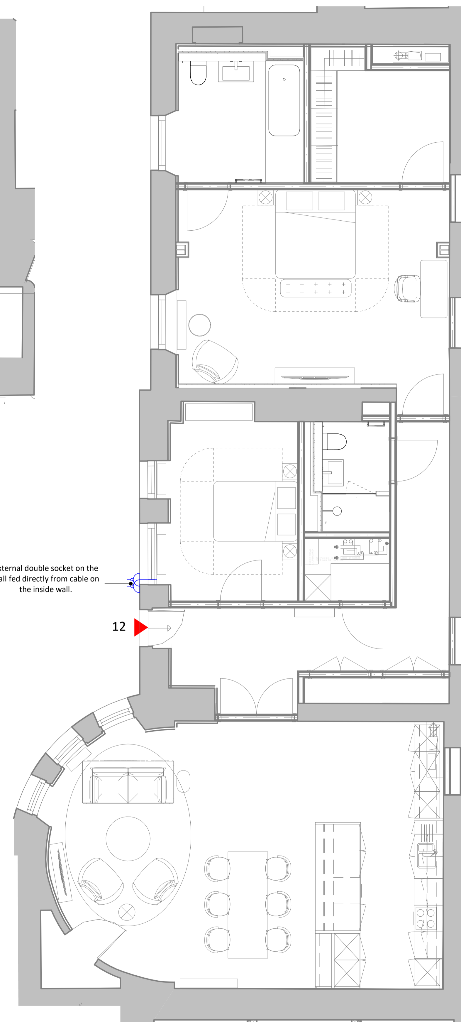
2 FT12 - LGF - Proposed Small Power Plan 1 : 50
