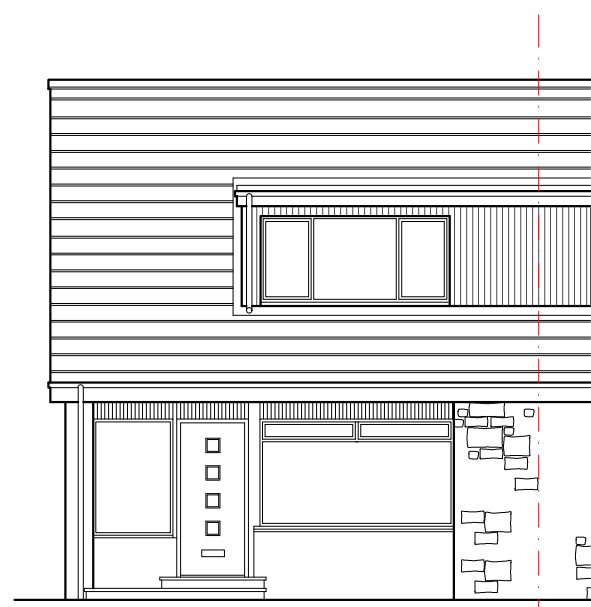
EAST ELEVATION
