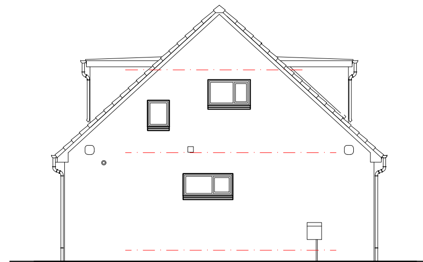
NORTH ELEVATION
