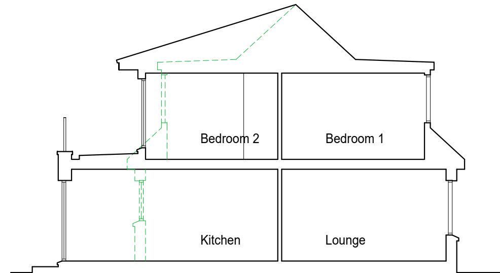
CROSS SECTION
