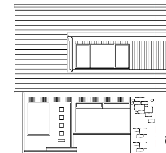
EAST ELEVATION No change to this elevation
