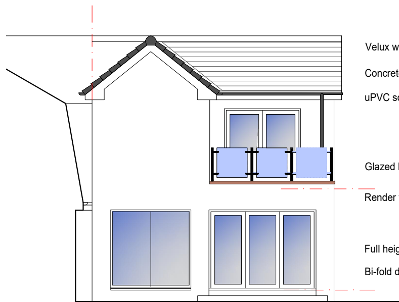
WEST ELEVATION
