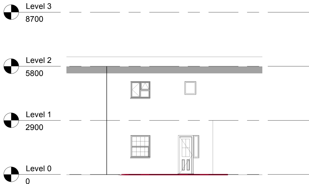
4 Rear Elevation 1 : 100
