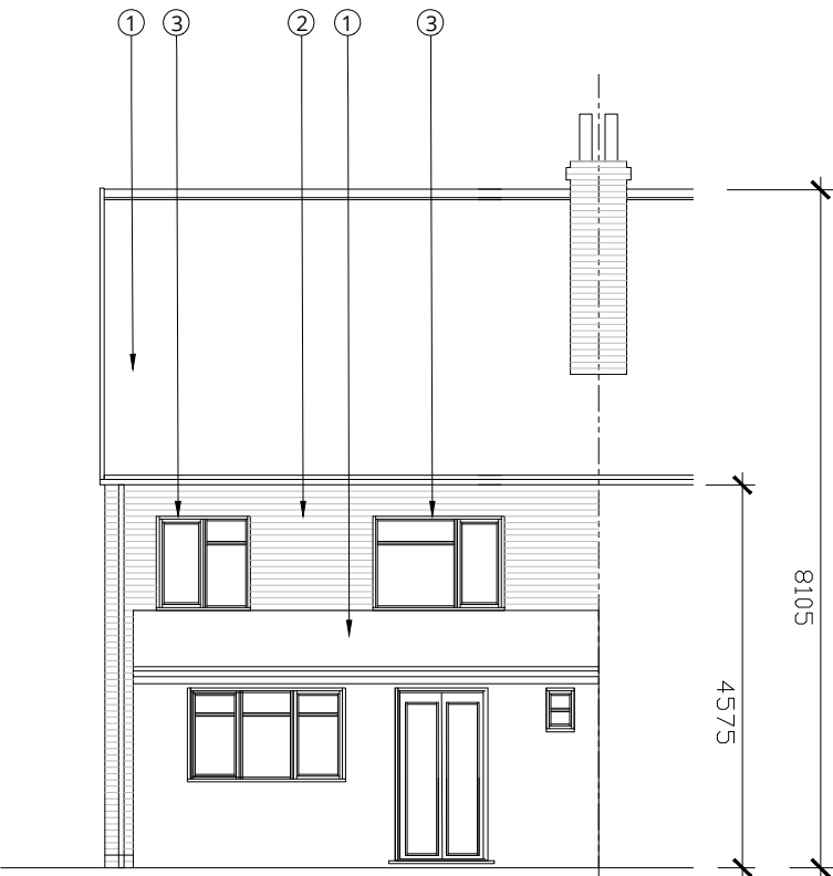
EAST ELEVATION (REAR)
