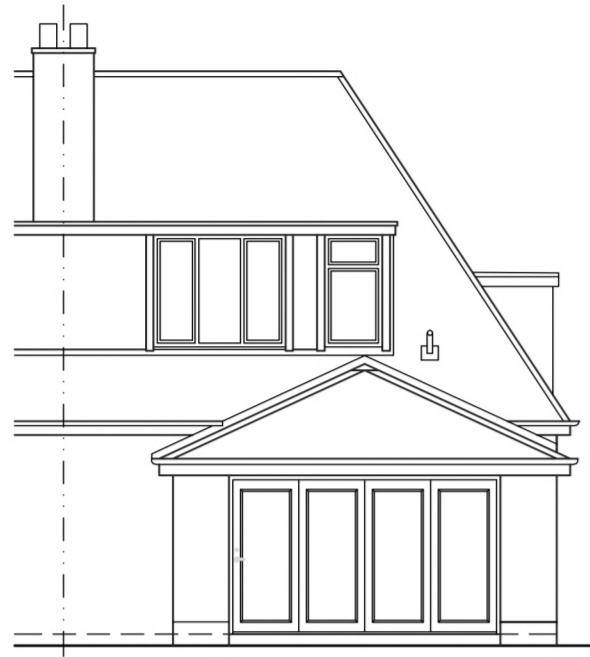
Rear North Elevation
